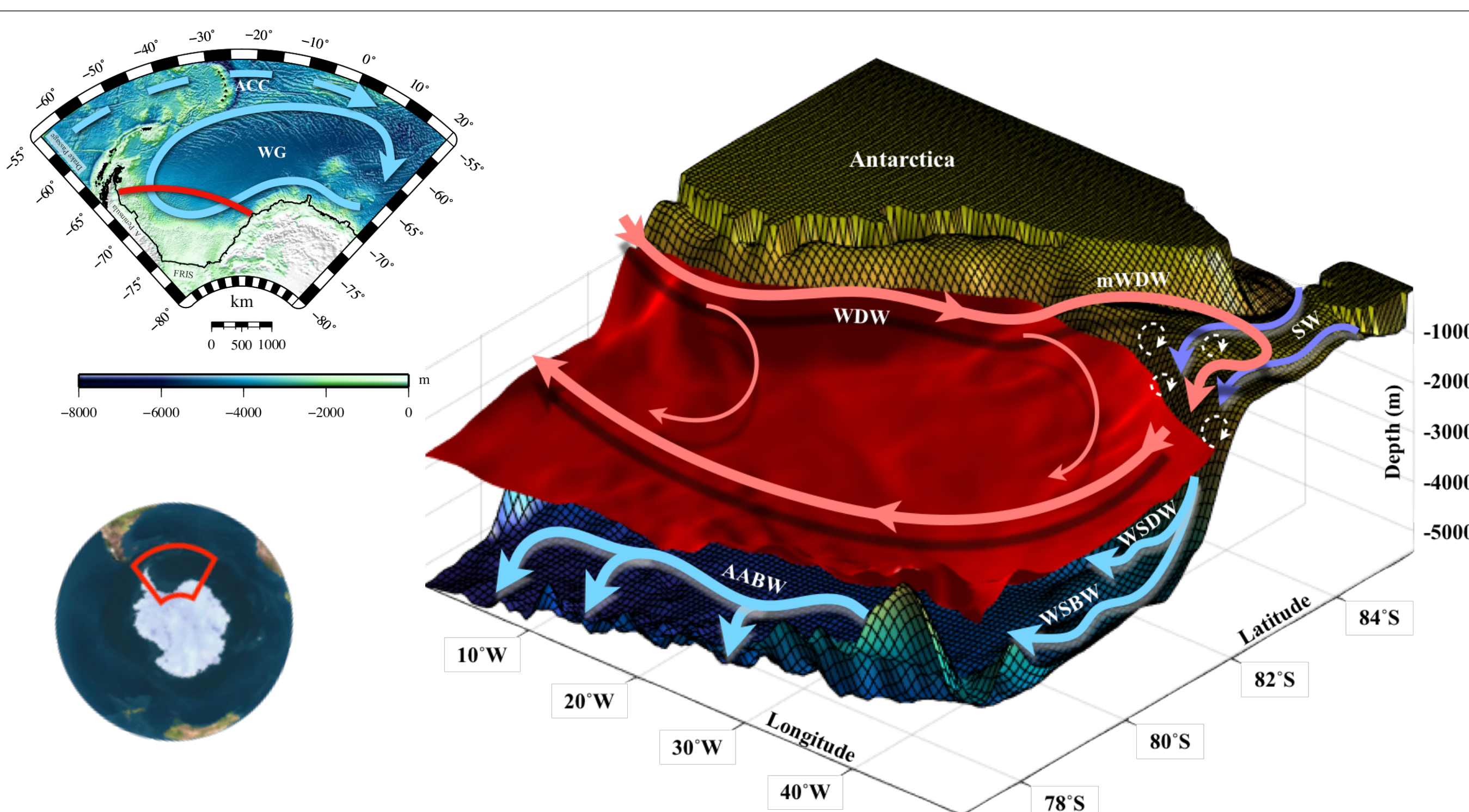
Perspective of the Weddell Sea multi-layer circulation, depicting the near-shelf break interactions between the Warm Deep Water and the super cooled Shelf Waters to form the Antarctic Bottom Water.
