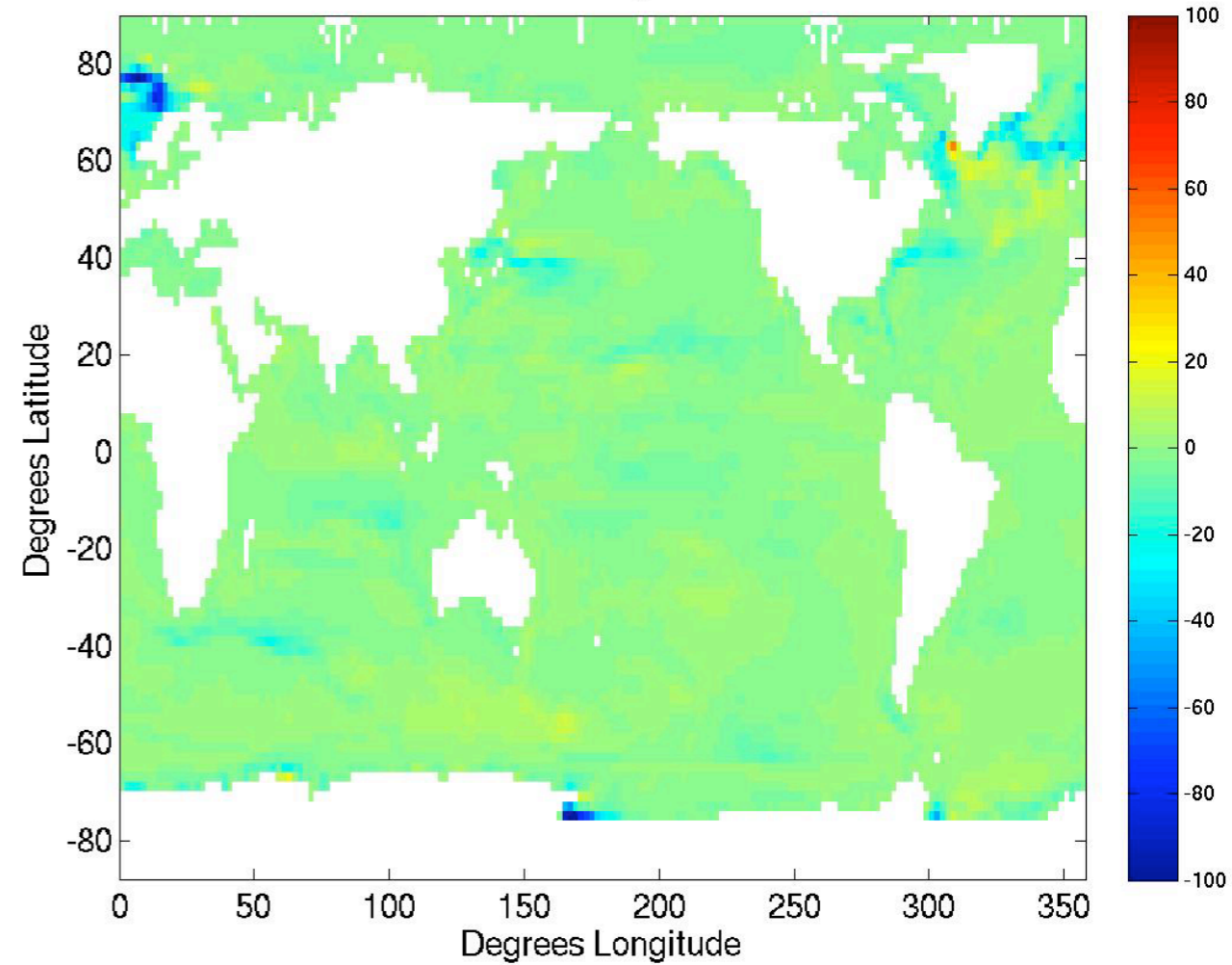
GOLD/CM2.2 MLD change due to MLE OND
