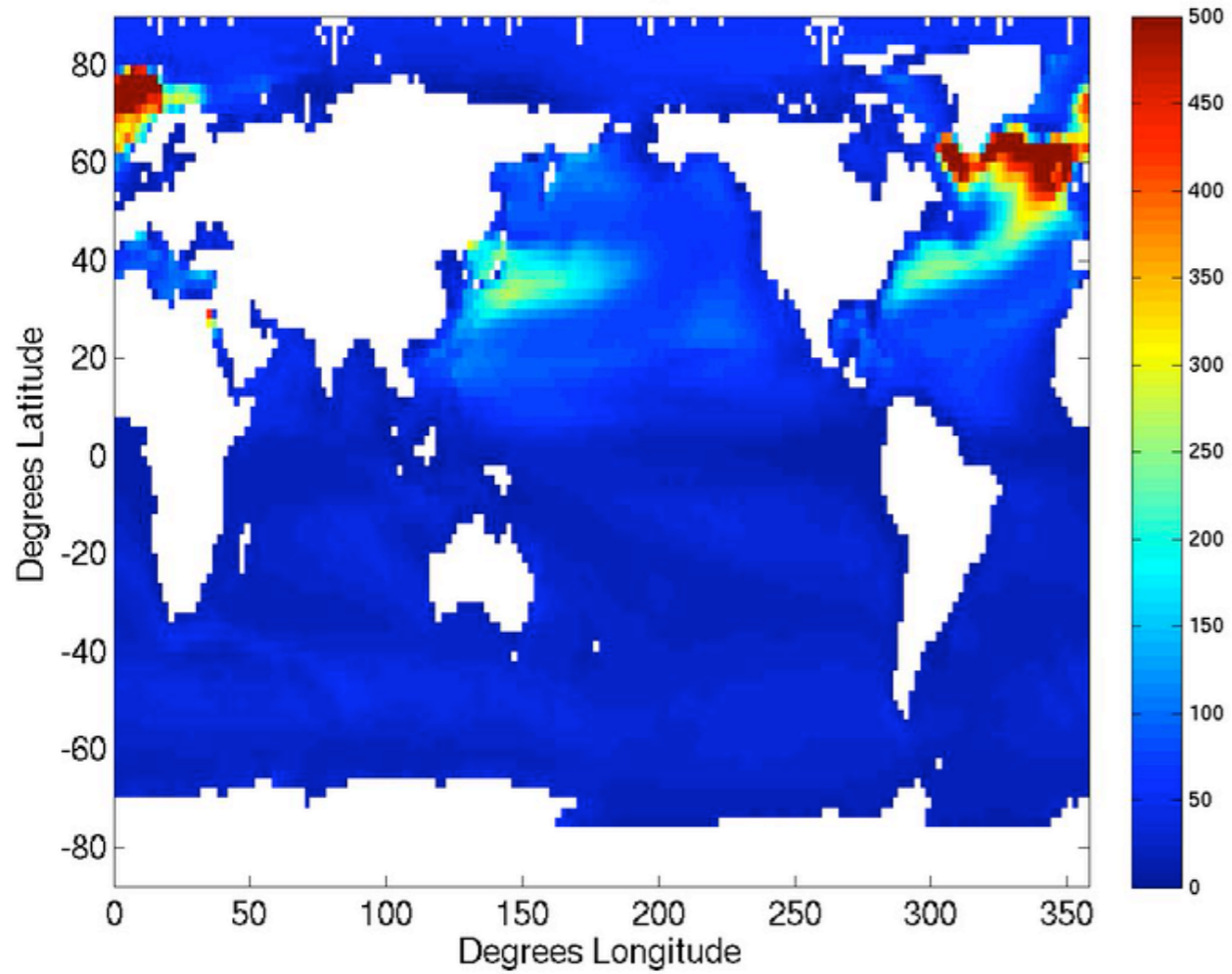
GOLD/CM2.2 with MLE param. BLT JFM
