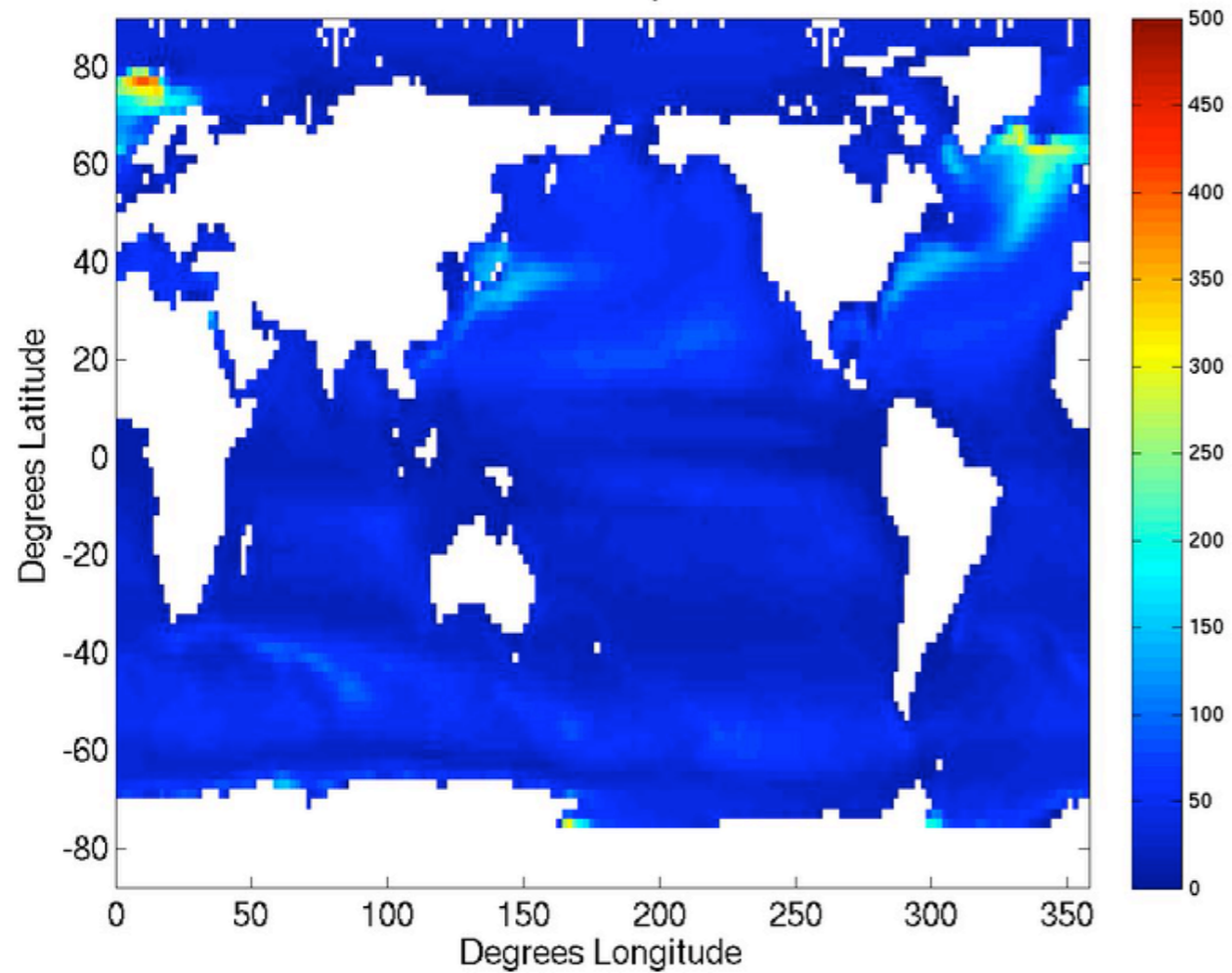
GOLD/CM2.2 with MLE param. BLT OND
