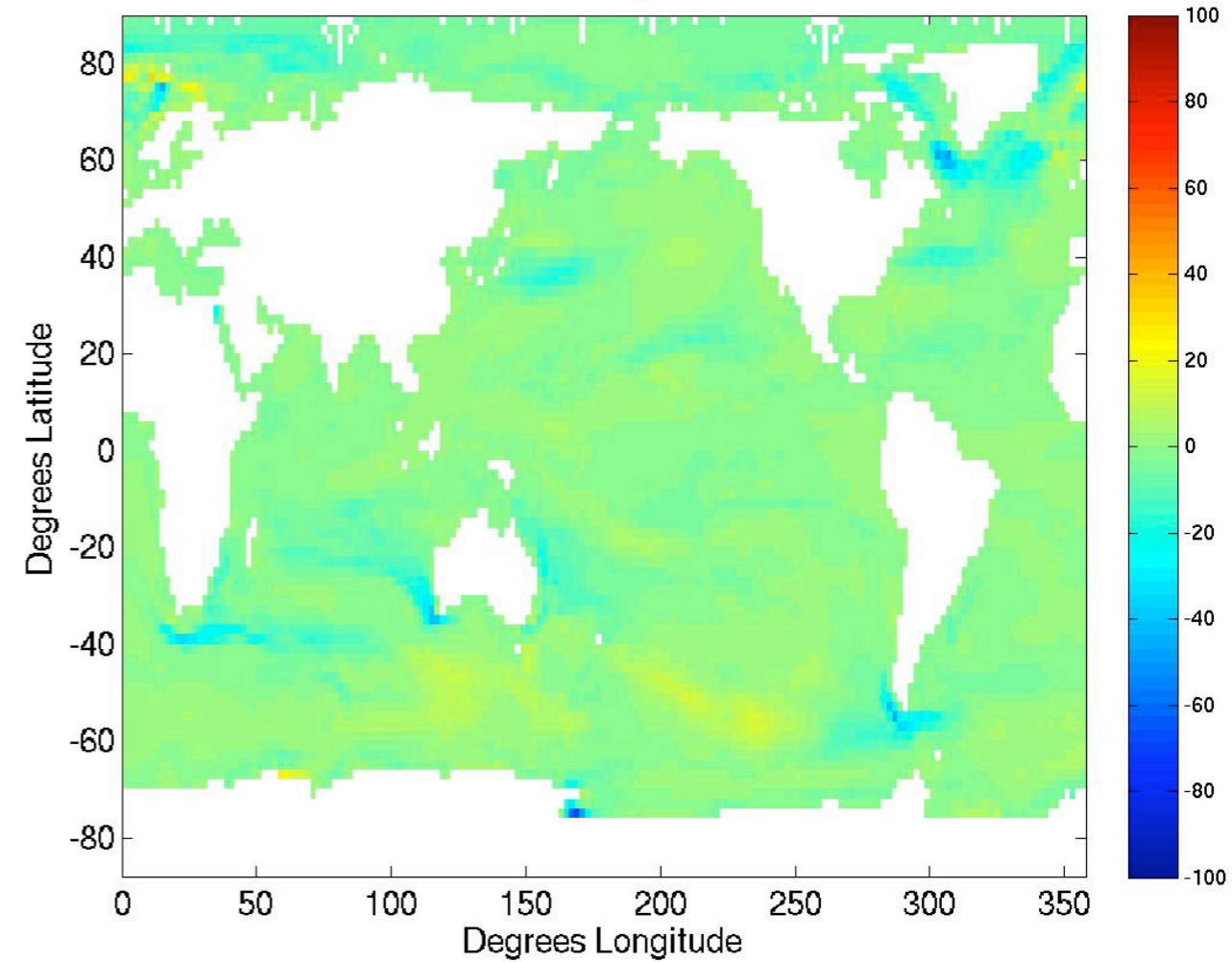
GOLD/CM2.2 MLD change due to MLE AMJ
