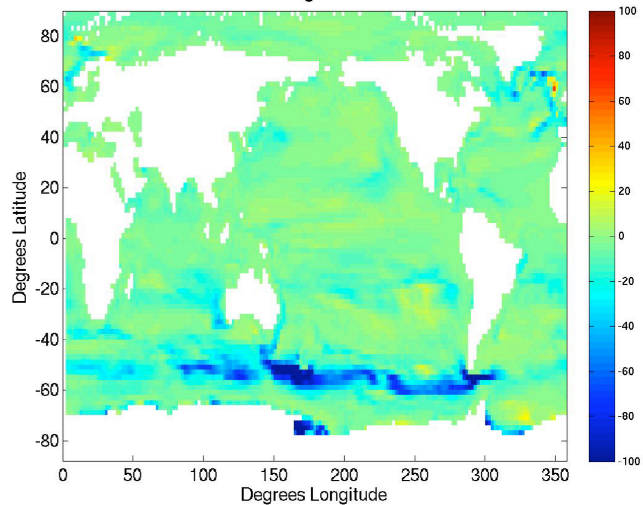
CCSM MLD change due to MLE OND
