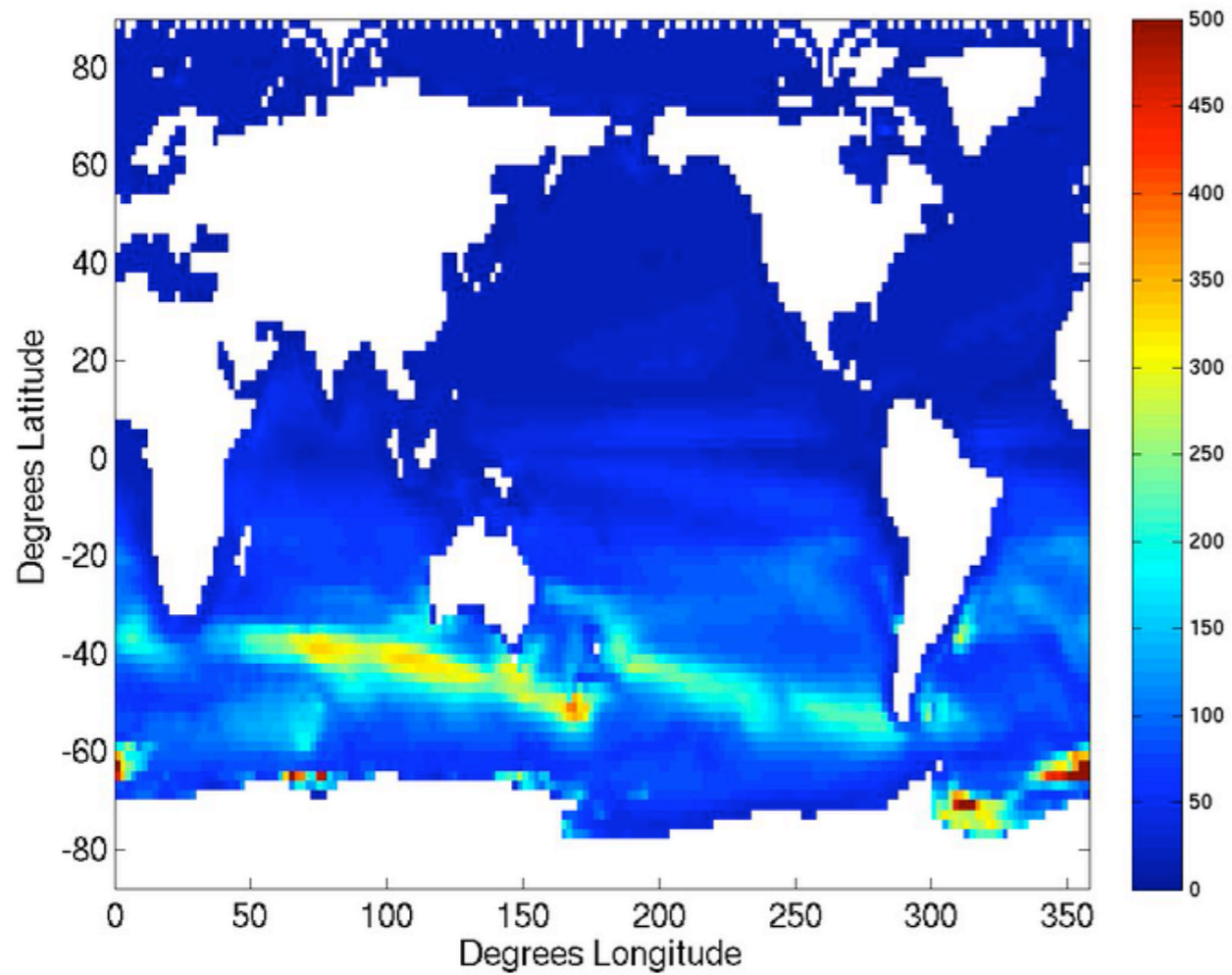
MOM/CM2.2 Control MLD JAS
