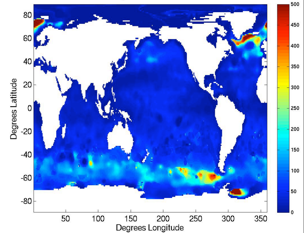
Monterey and Levitus MLD AMJ
