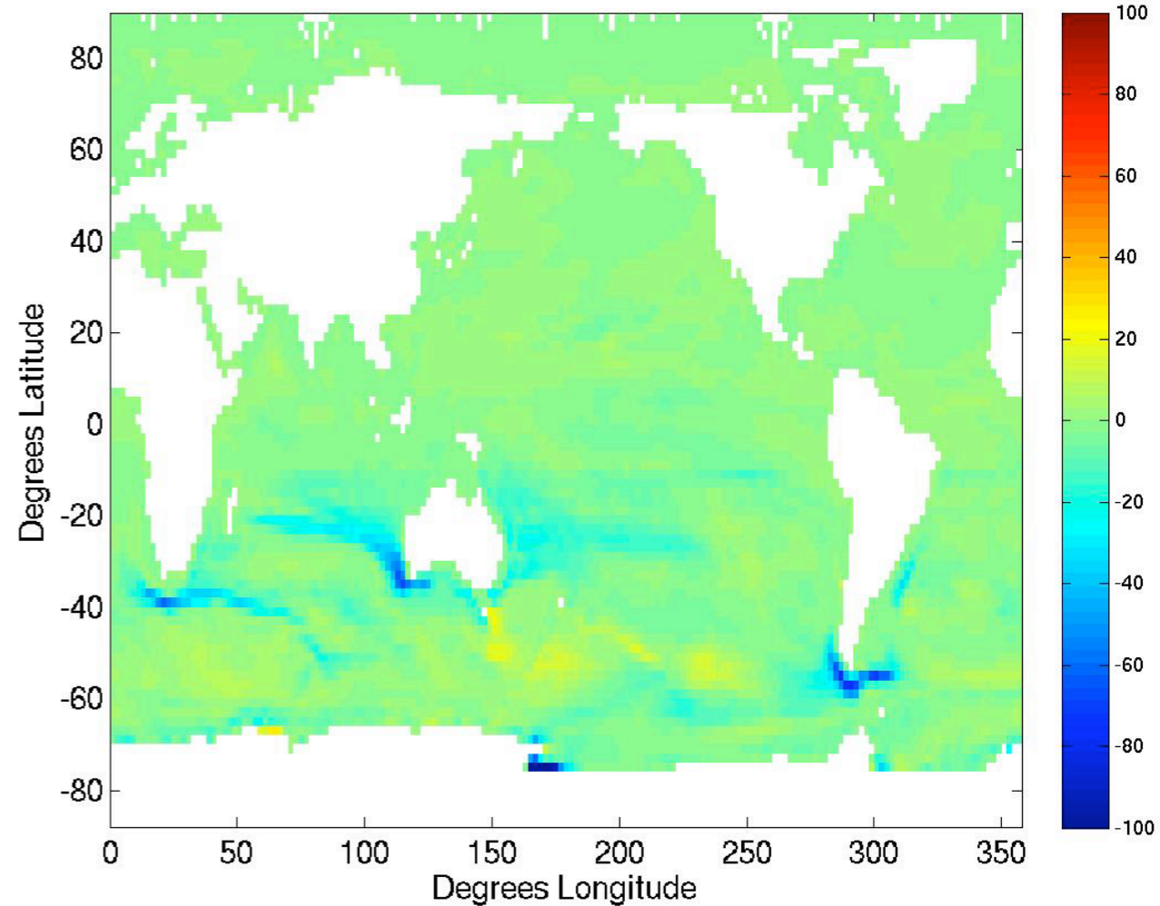
GOLD/CM2.2 MLD change due to MLE JAS
