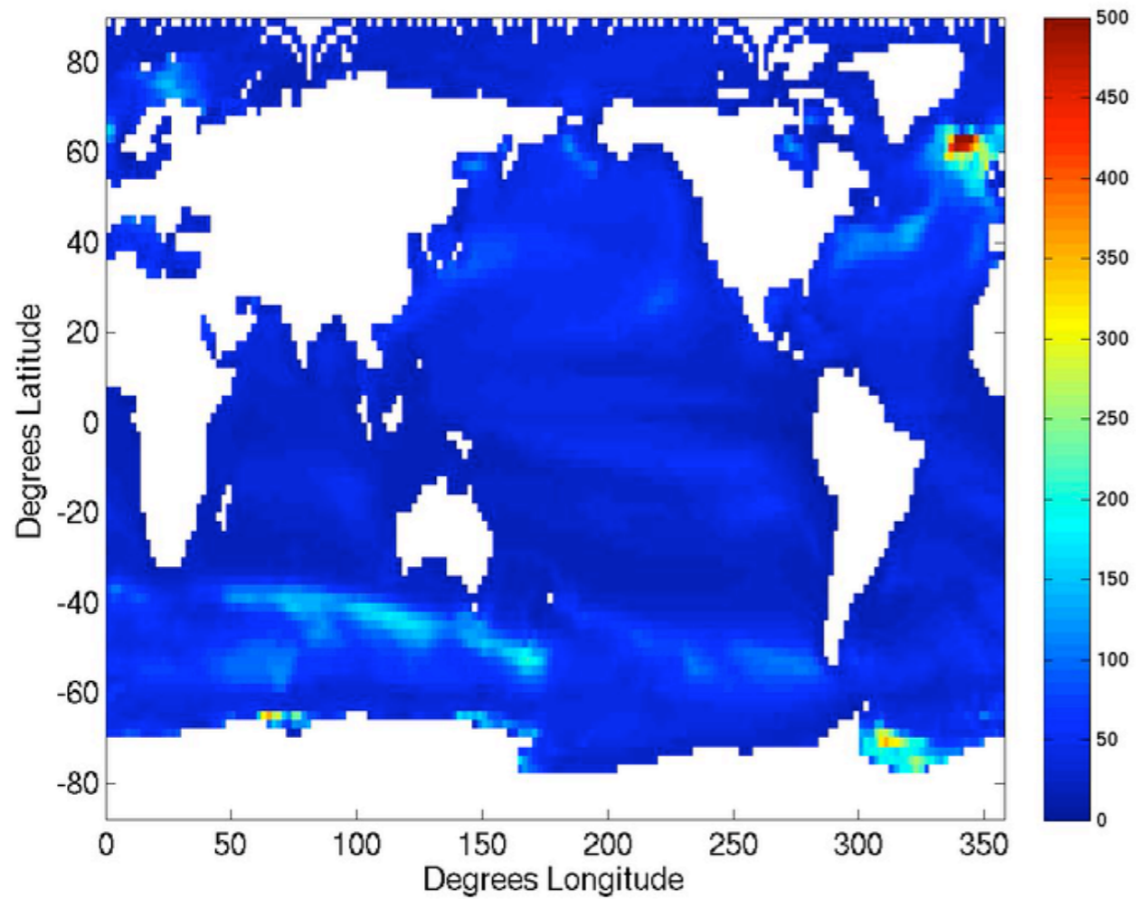
MOM/CM2.2 Control MLD OND
