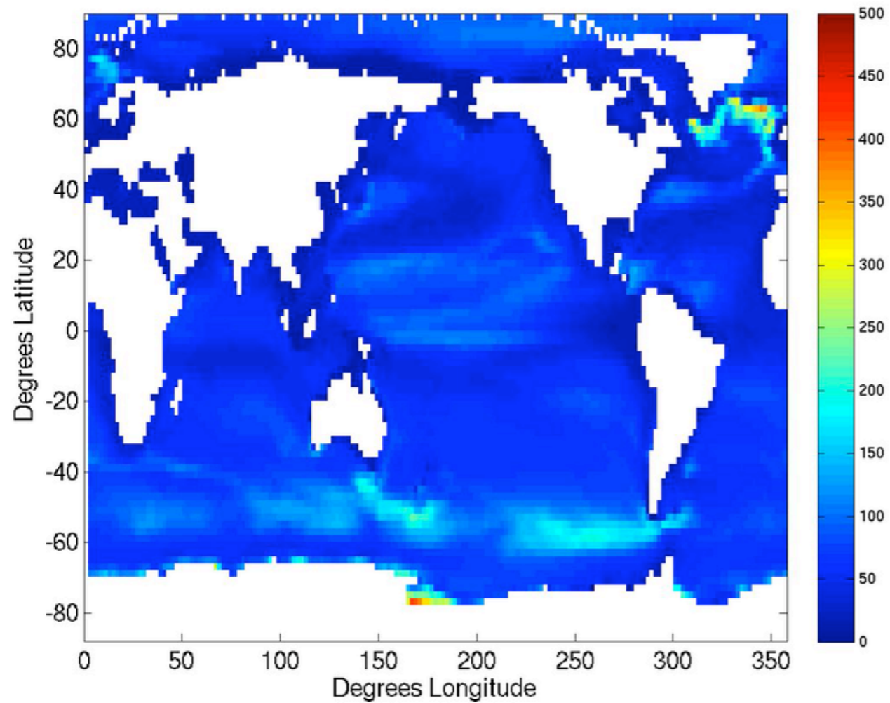
CCSM Control MLD AMJ
