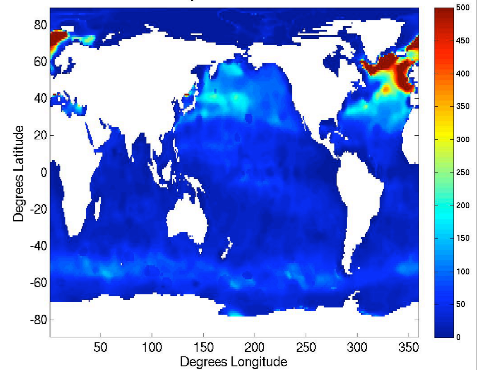
Monterey and Levitus MLD JFM
