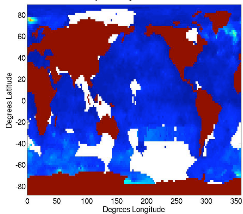
de Boyer-Montegut et al. MLD AMJ
