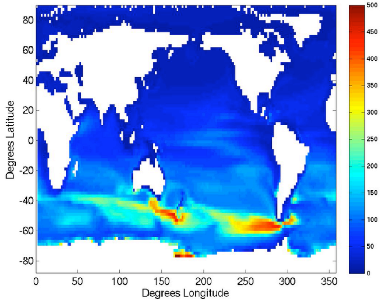
CCSM Control MLD JAS
