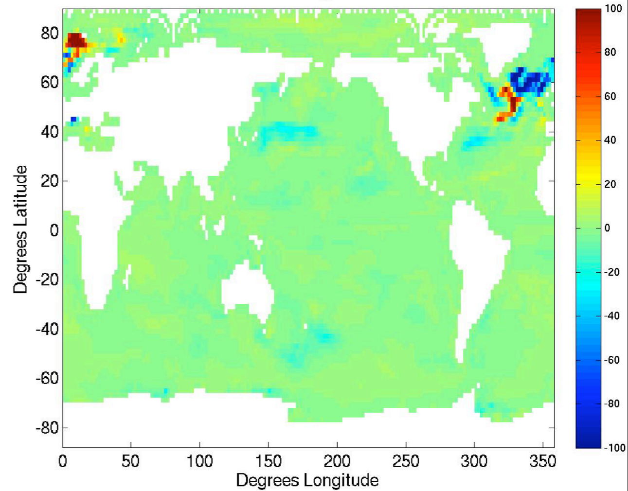
MOM/CM2.2 MLD change due to MLE AMJ
