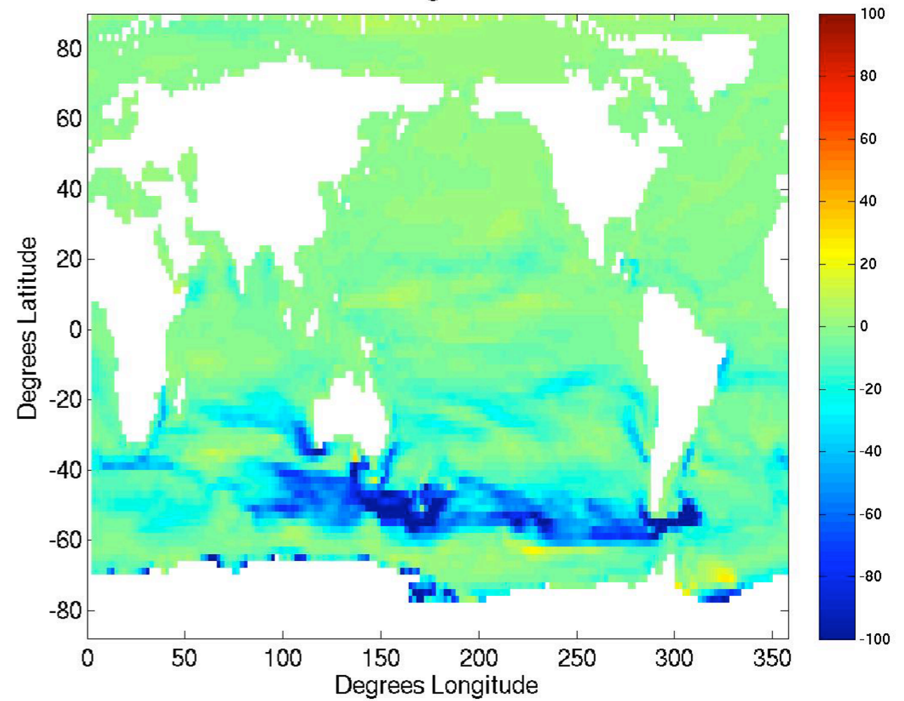
CCSM MLD change due to MLE JAS
