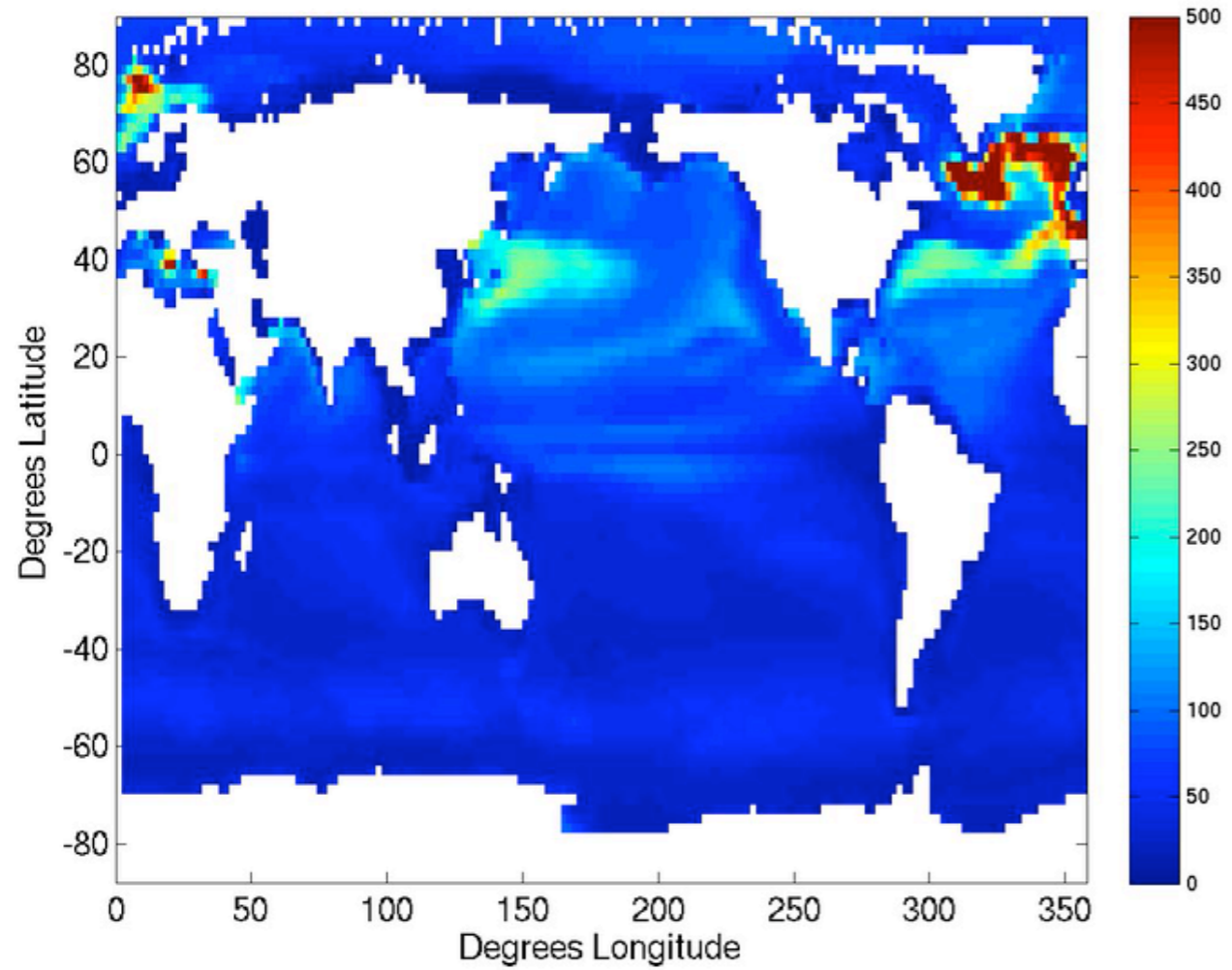
CCSM Control MLD JFM
