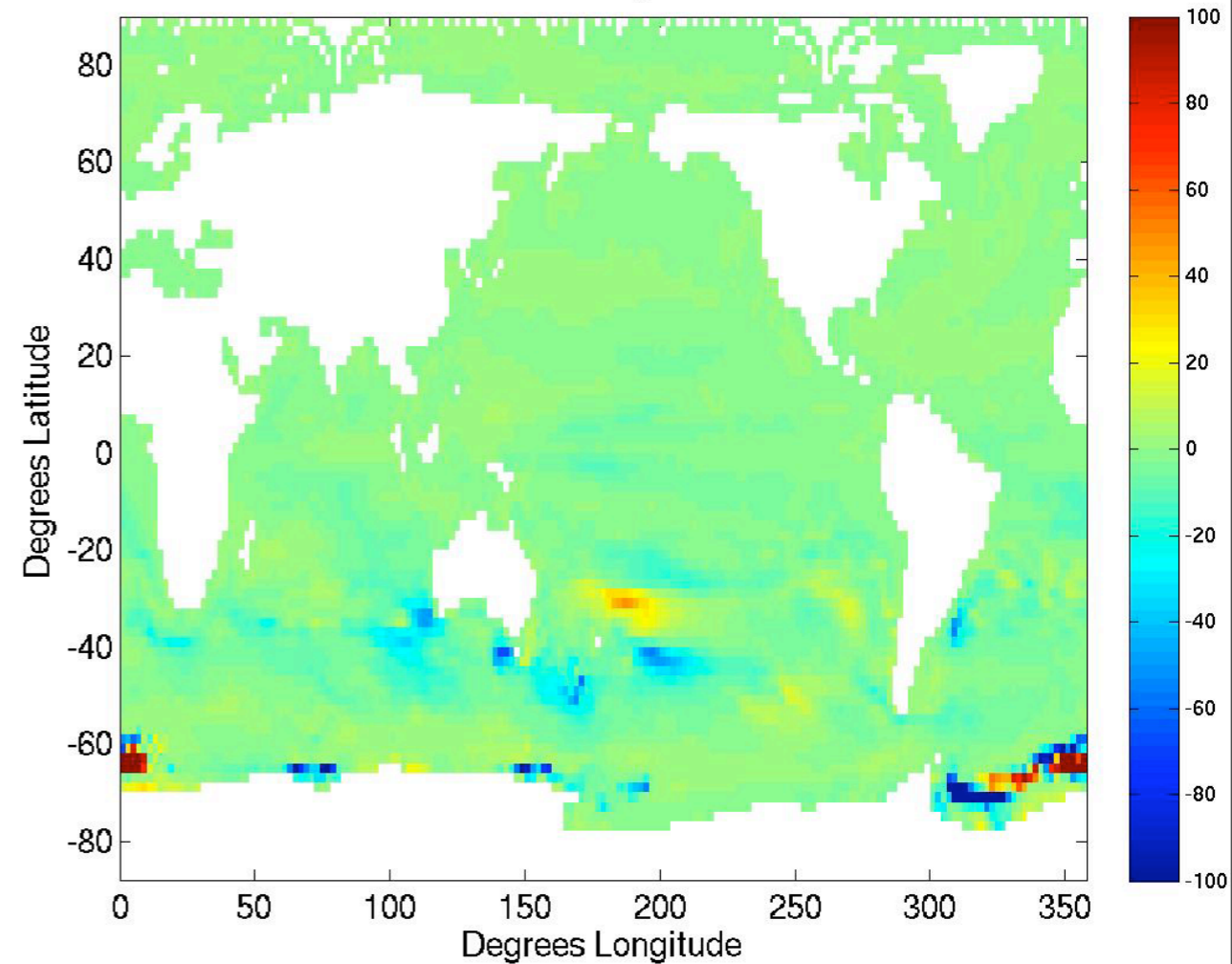
MOM/CM2.2 MLD change due to MLE JAS
