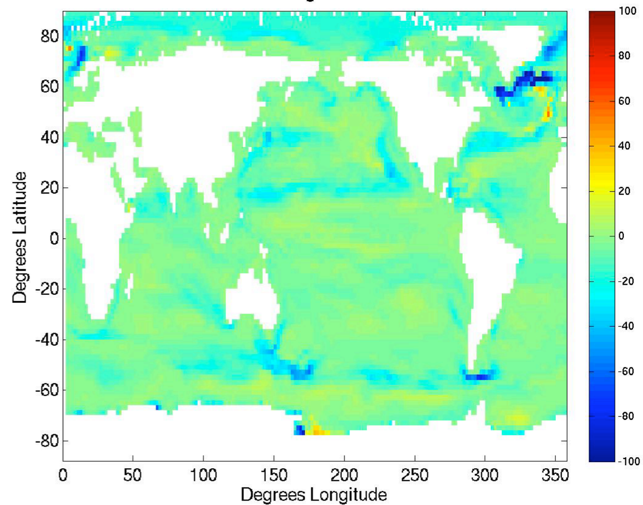
CCSM MLD change due to MLE AMJ
