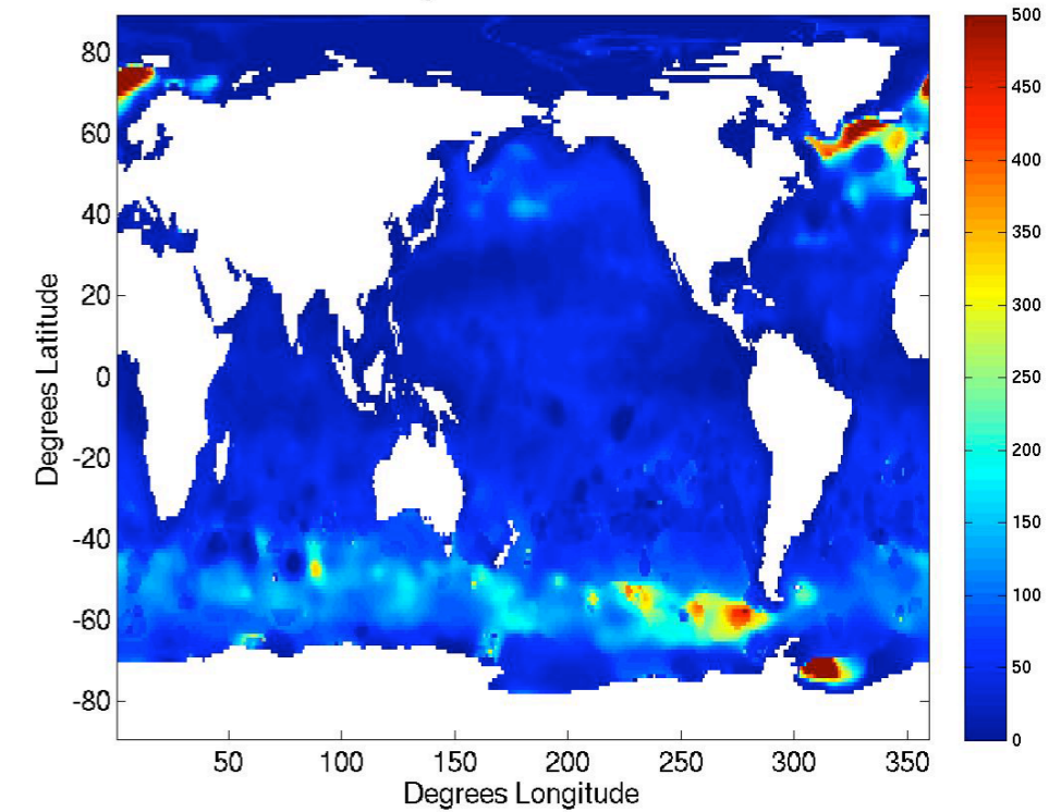
Monterey and Levitus MLD AMJ
