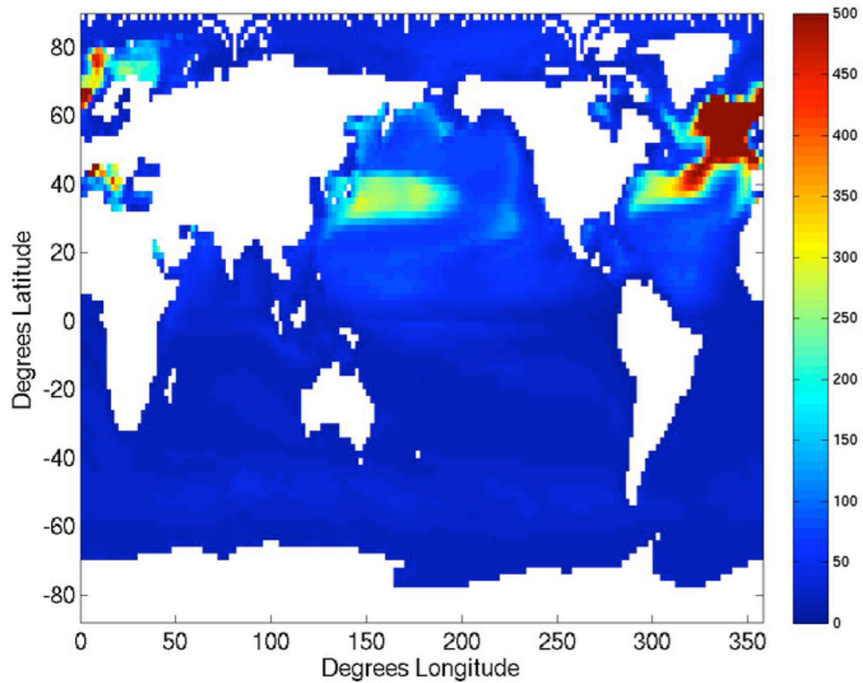
MOM/CM2.2 Control MLD JFM
