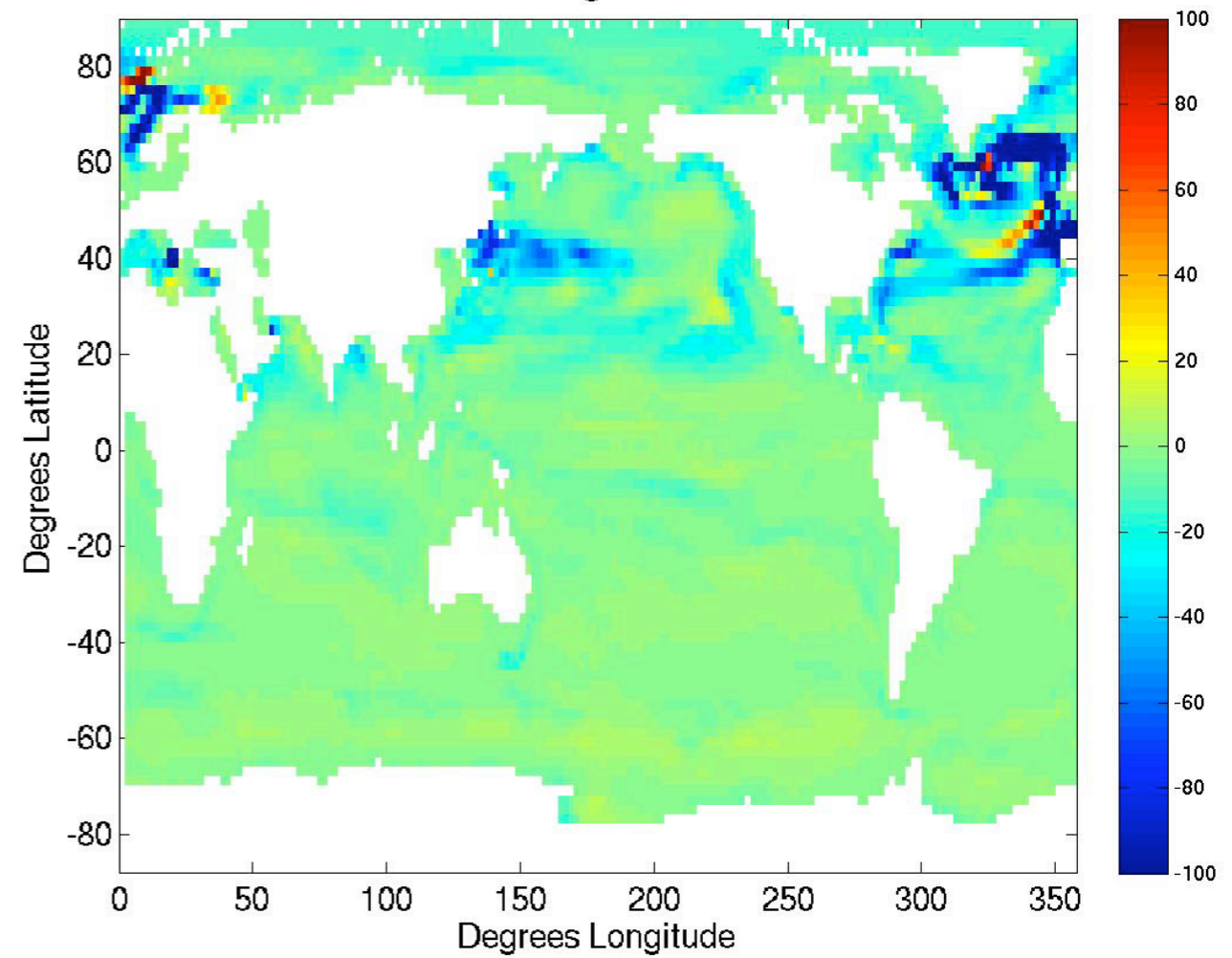
CCSM MLD change due to MLE JFM
