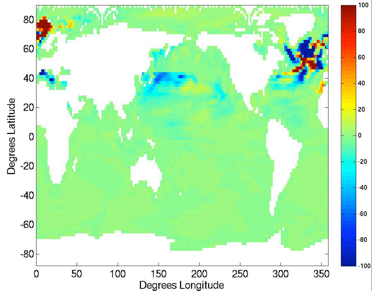
MOM/CM2.2 MLD change due to MLE JFM
