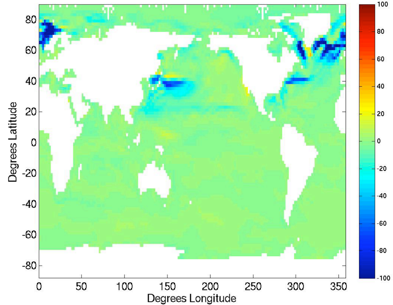
GOLD/CM2.2 MLD change due to MLE JFM
