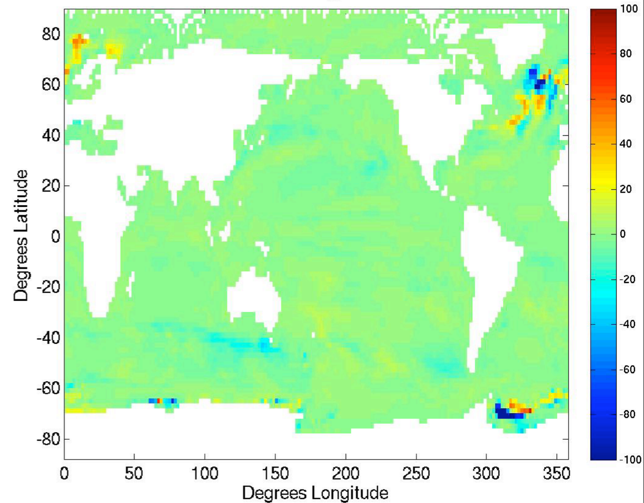
MOM/CM2.2 MLD change due to MLE OND
