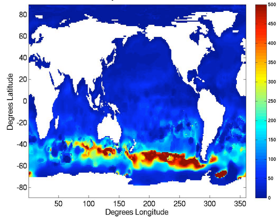
Monterey and Levitus MLD JAS
