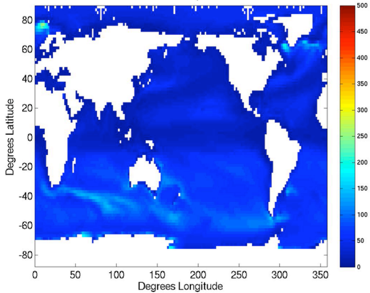
GOLD/CM2.2 with MLE param. BLT AMJ
