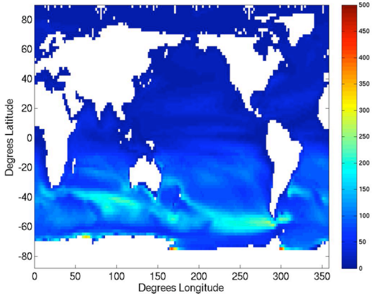
GOLD/CM2.2 with MLE param. BLT JAS
