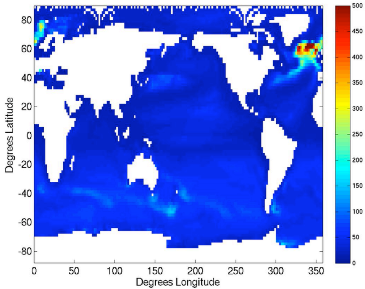
MOM/CM2.2 Control MLD AMJ
