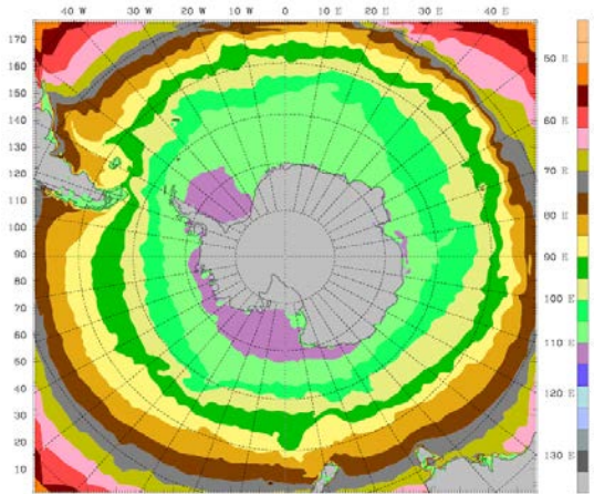
Annual-mean SST
