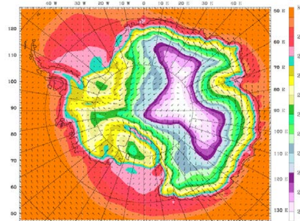
JJA 2-m T + 10-m Winds
