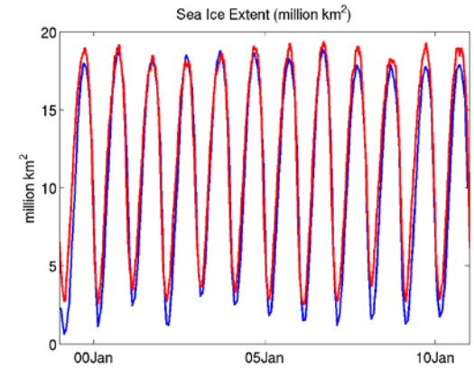
Sea Ice Extent
