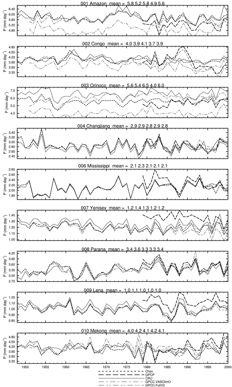
FIG. 1. Time series of annual precipitation averaged over world's major river basins based on five observational datasets: Chen et al. (2002), GPCP, CRU, and GPCP fixed-station (VASclimO) and all-station (FullV3) products. Also shown on the top of each panel are long-term means of these products in the above order.
