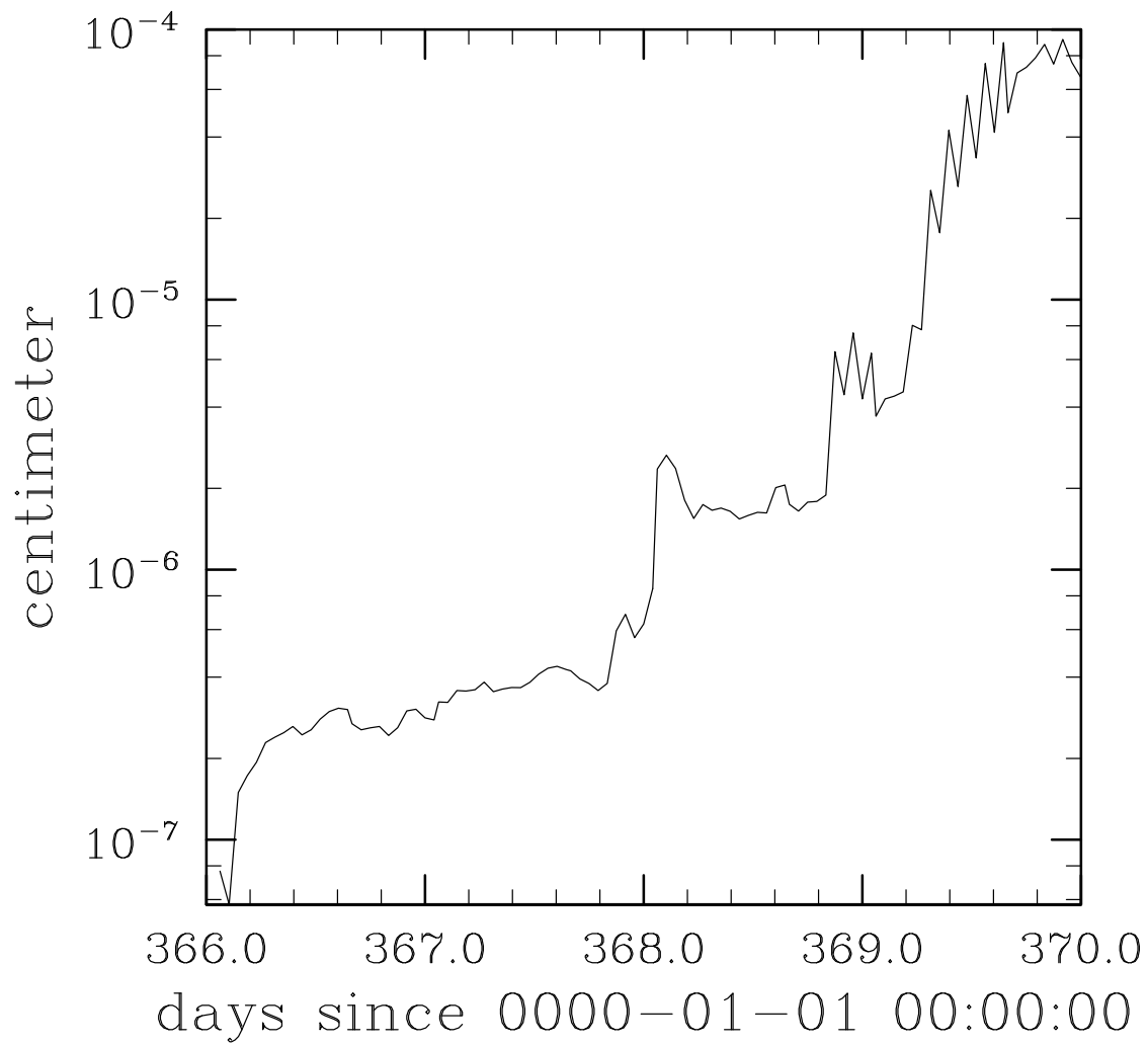
RMS Diff SSH Case1 vs Case3 bluefire
