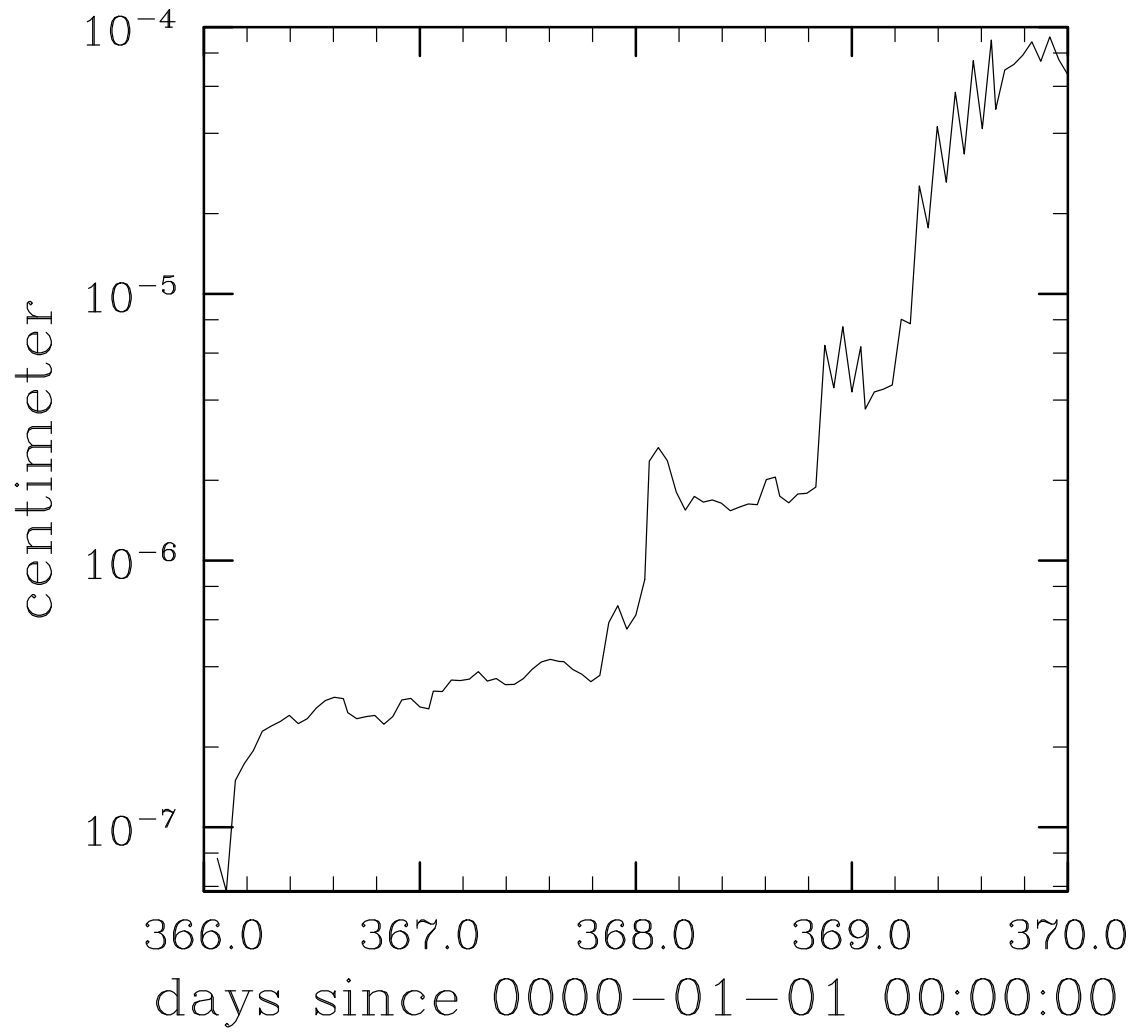
RMS Diff SSH Case1 vs Case3 jaguar
