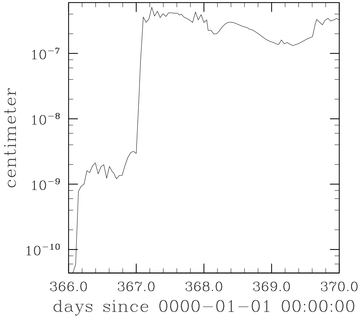
RMS Diff SSH Case2 bluefire vs jaguar
