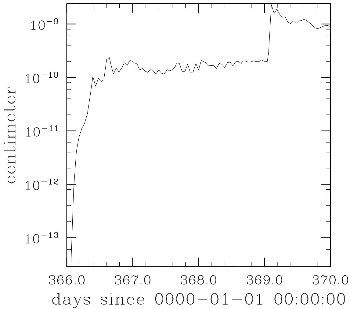
RMS Diff SSH Case4 vs Case5 jaguar
