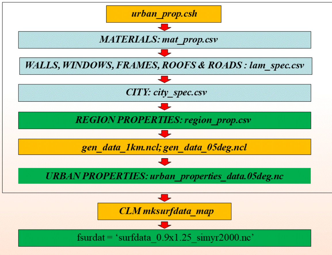
Figure 15.3: Schematic of THESIS urban properties tool. Executable scripts are in orange, input files are blue, and output files are green. Items within the black box outline are either read in as input, executed, or output by the driver script (urban_prop.csh).
