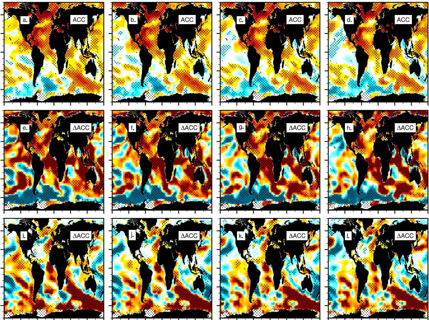
ACC, Sea Surface Temperature, OBS=ERSSTv5, Season=JAS, (LY 1-5: 1957.6-2014.6), detrended LY 1-5 LY 2-6 LY 3-7 LY 4-8
