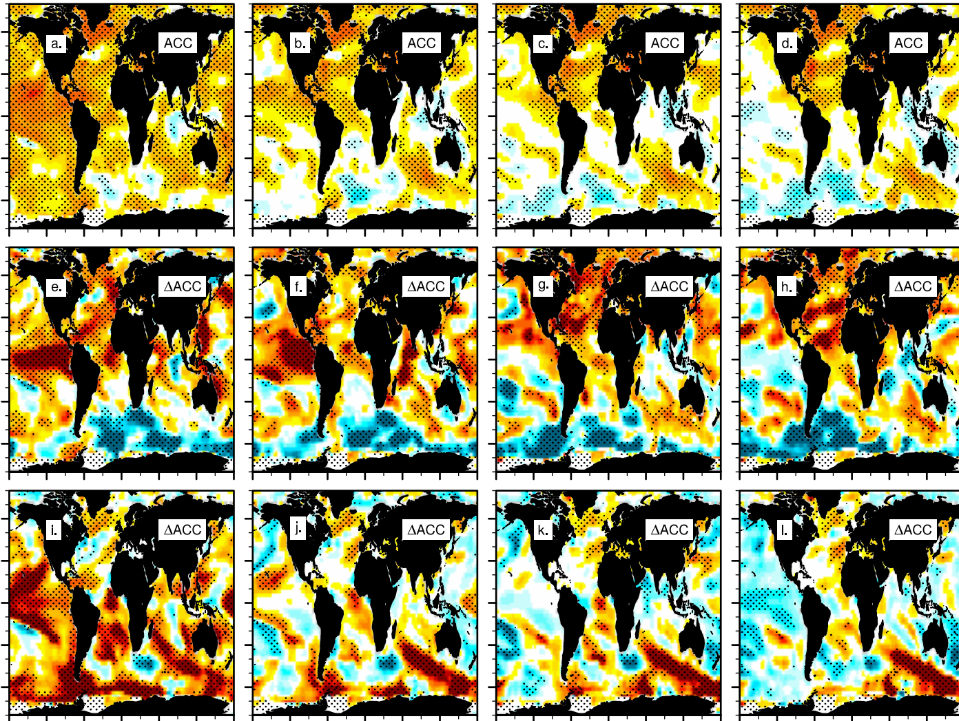
ACC, Sea Surface Temperature, OBS=ERSSTv5, Season=JAS, (LY 1: 1955.6-2016.6), detrended
