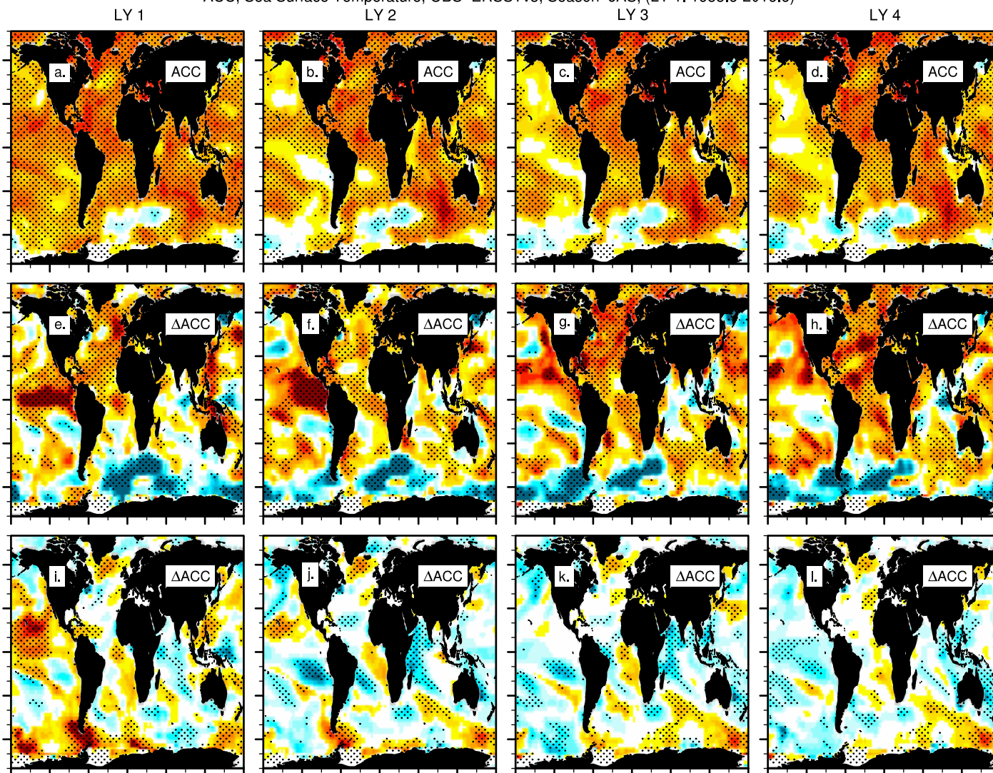
ACC, Sea Surface Temperature, OBS=ERSSTv5, Season=JAS, (LY 1: 1955.6-2016.6)
