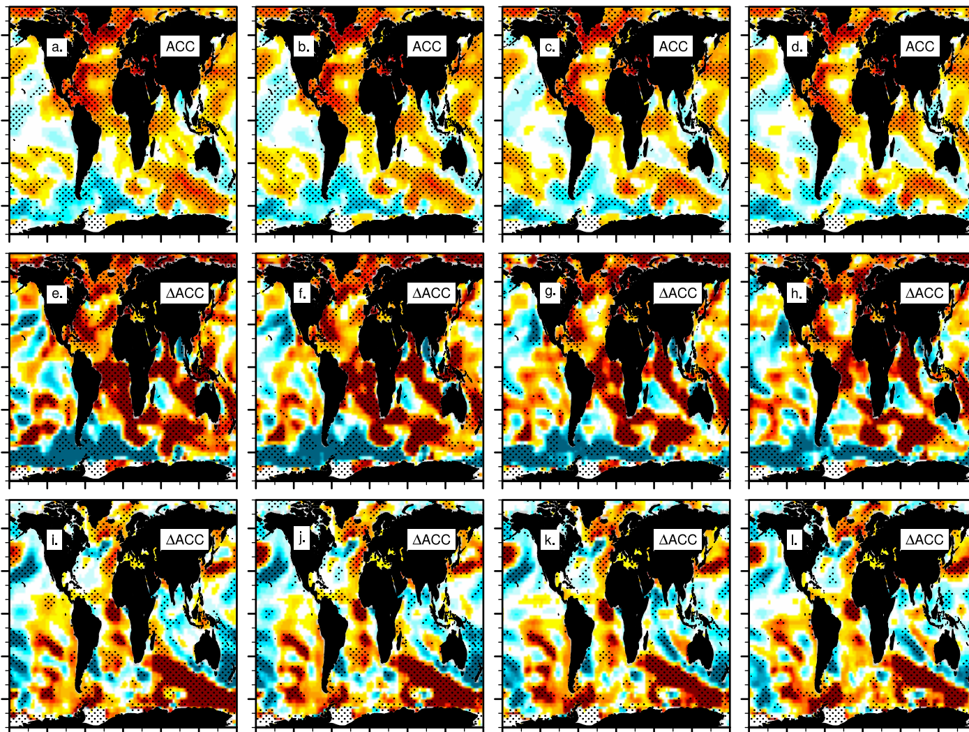
ACC, Sea Surface Temperature, OBS=ERSSTv5, Season=JAS, (LY 3-7: 1959.6-2014.6), detrended LY 3-7 LY 4-8 LY 5-9 LY 6-10
