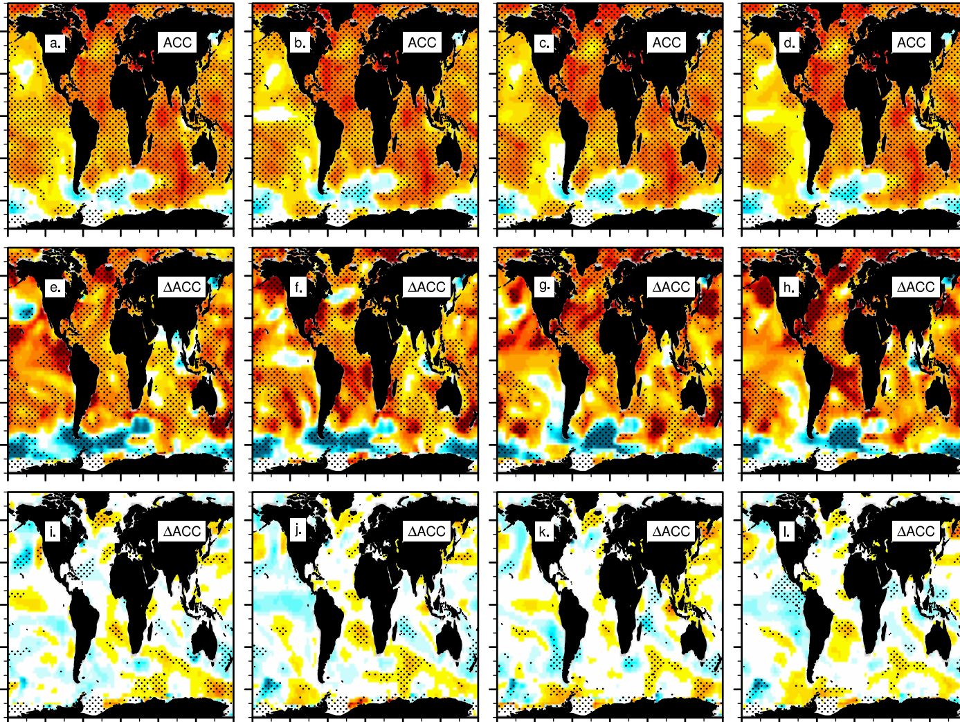
ACC, Sea Surface Temperature, OBS=ERSSTv5, Season=JAS, (LY 5: 1959.6-2016.6)
