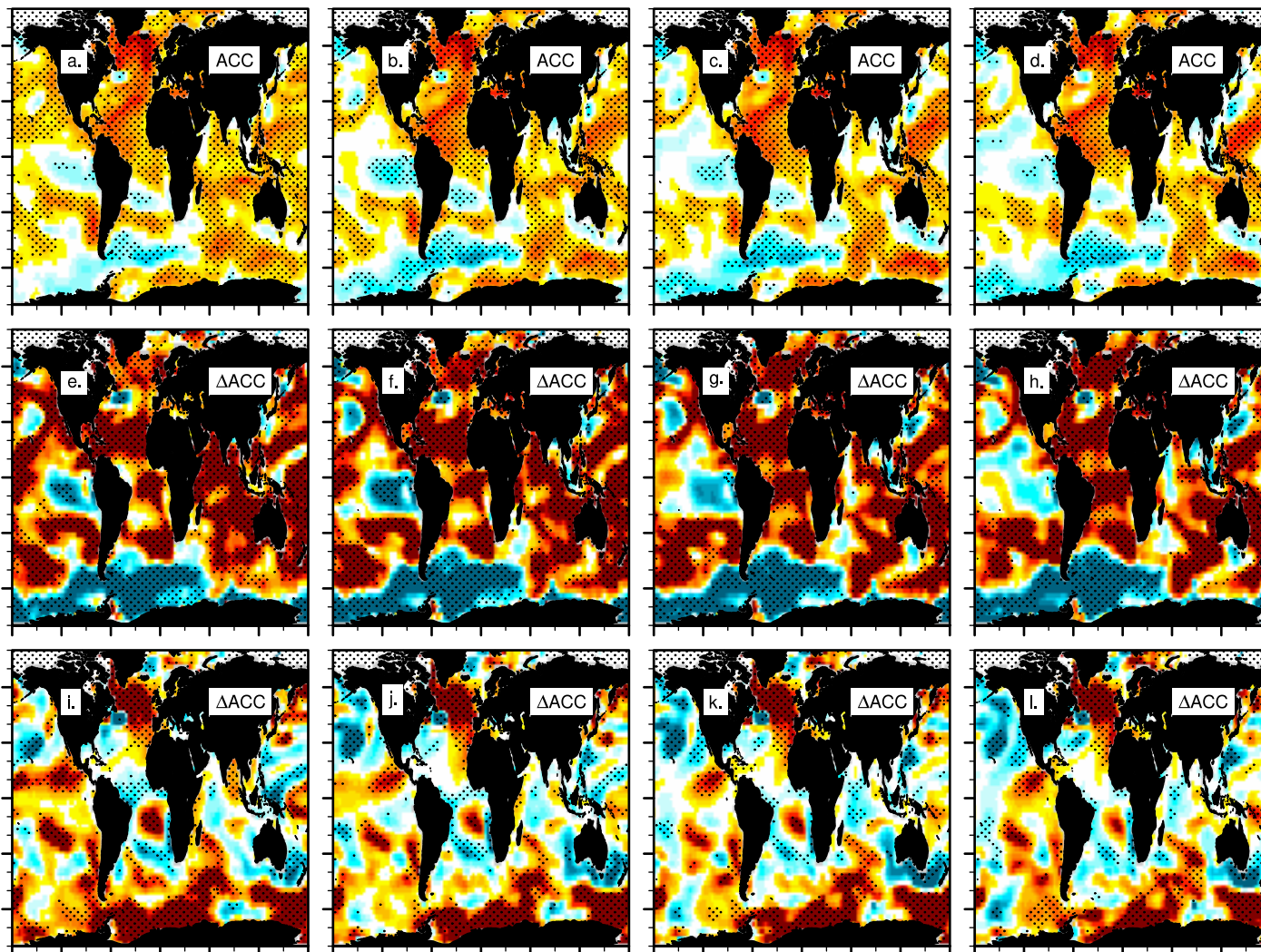
ACC, Sea Surface Temperature, OBS=ERSSTv5, Season=JFM, (LY 1-5: 1957.1-2014.1), detrended LY 1-5 LY 2-6 LY 3-7 LY 4-8
