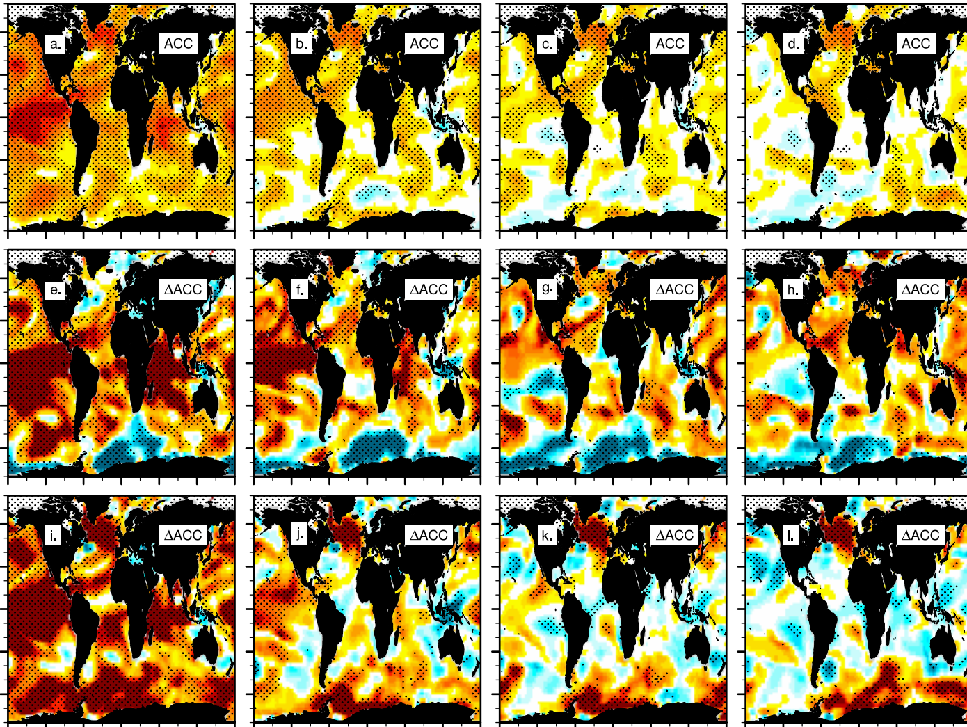
ACC, Sea Surface Temperature, OBS=ERSSTv5, Season=JFM, (LY 1: 1955.1-2016.1), detrended
