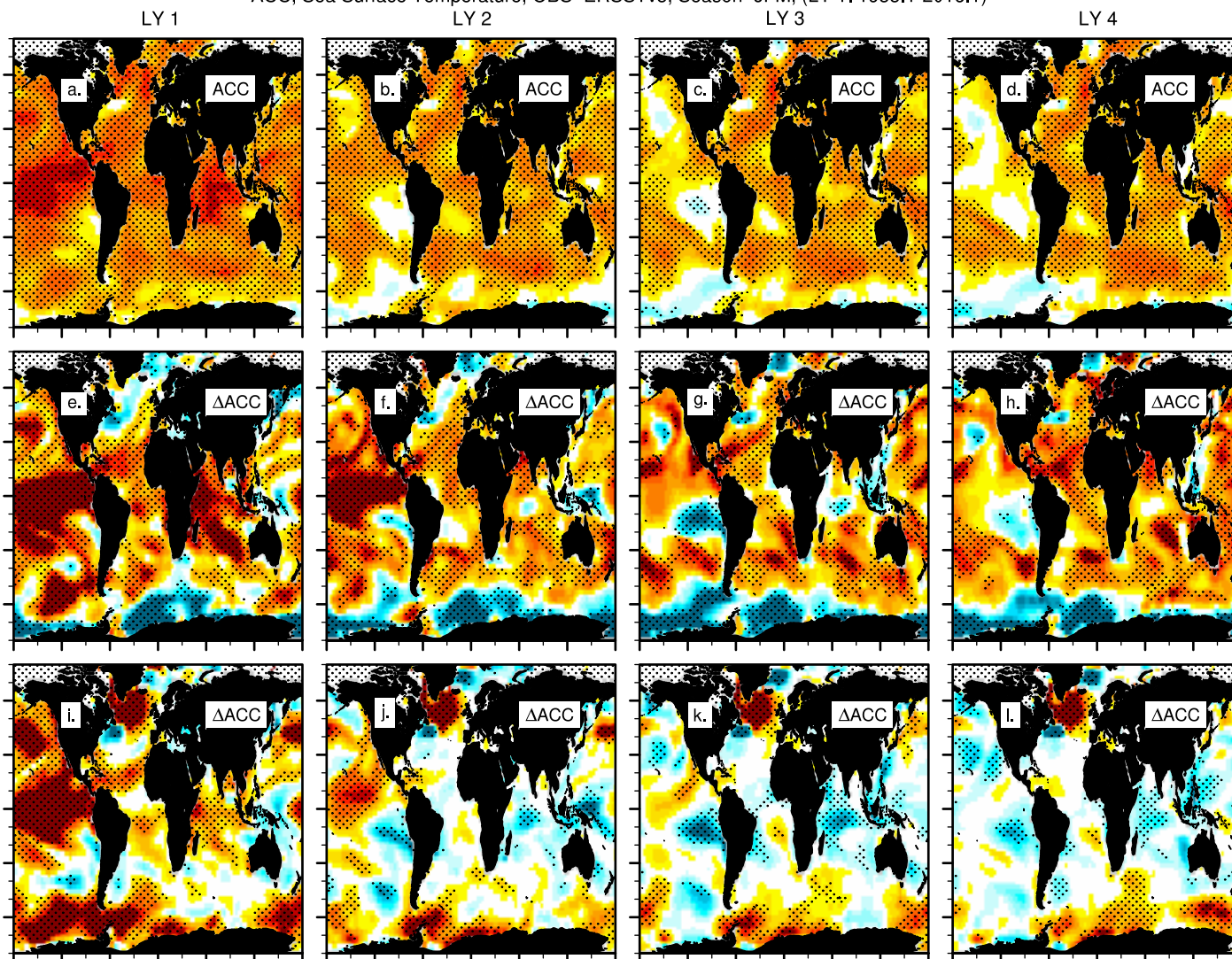
ACC, Sea Surface Temperature, OBS=ERSSTv5, Season=JFM, (LY 1: 1955.1-2016.1)
