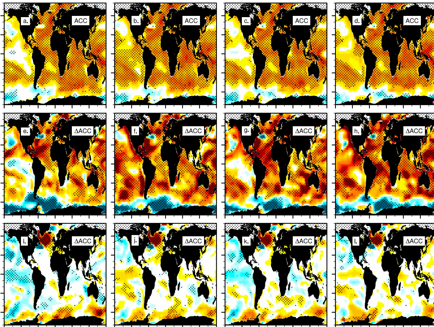
ACC, Sea Surface Temperature, OBS=ERSSTv5, Season=JFM, (LY 5: 1959.1-2016.1)
