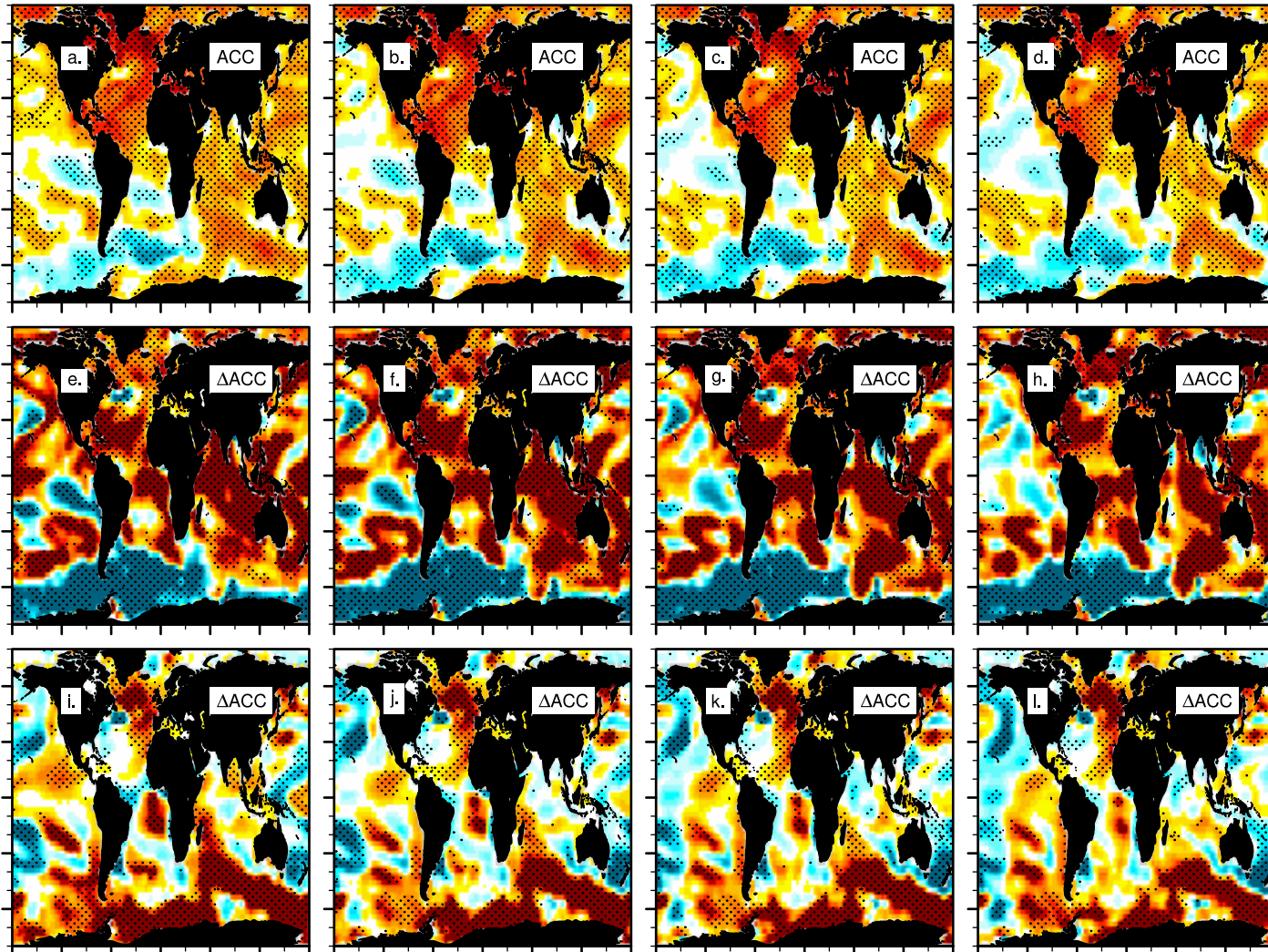
ACC, Sea Surface Temperature, OBS=ERSSTv5, Season=ANNUAL, (LY 1-5: 1957.5-2014.5), detrended LY 1-5 LY 2-6 LY 3-7 LY 4-8
