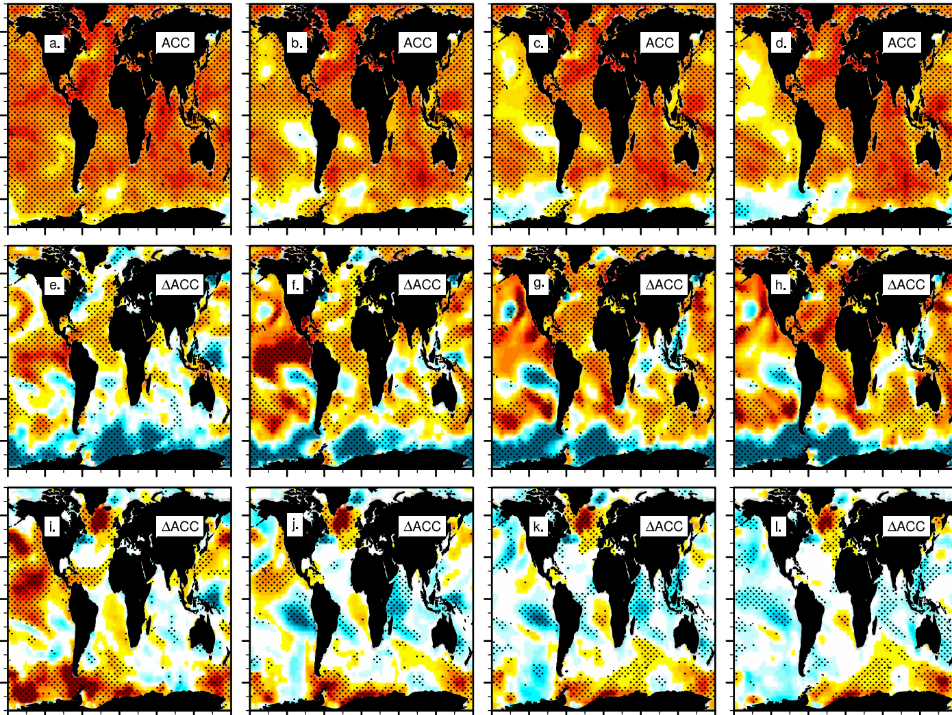
ACC, Sea Surface Temperature, OBS=ERSSTv5, Season=ANNUAL, (LY 1: 1955.5-2016.5)
