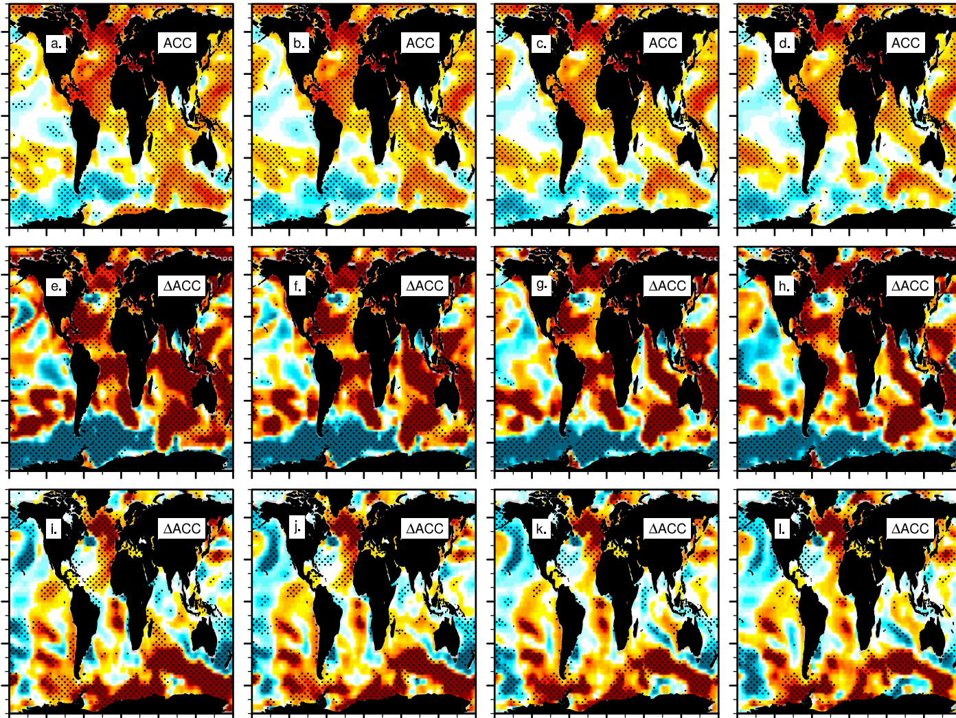
ACC, Sea Surface Temperature, OBS=ERSSTv5, Season=ANNUAL, (LY 3-7: 1959.5-2014.5), detrended LY 3-7 LY 4-8 LY 5-9 LY 6-10
