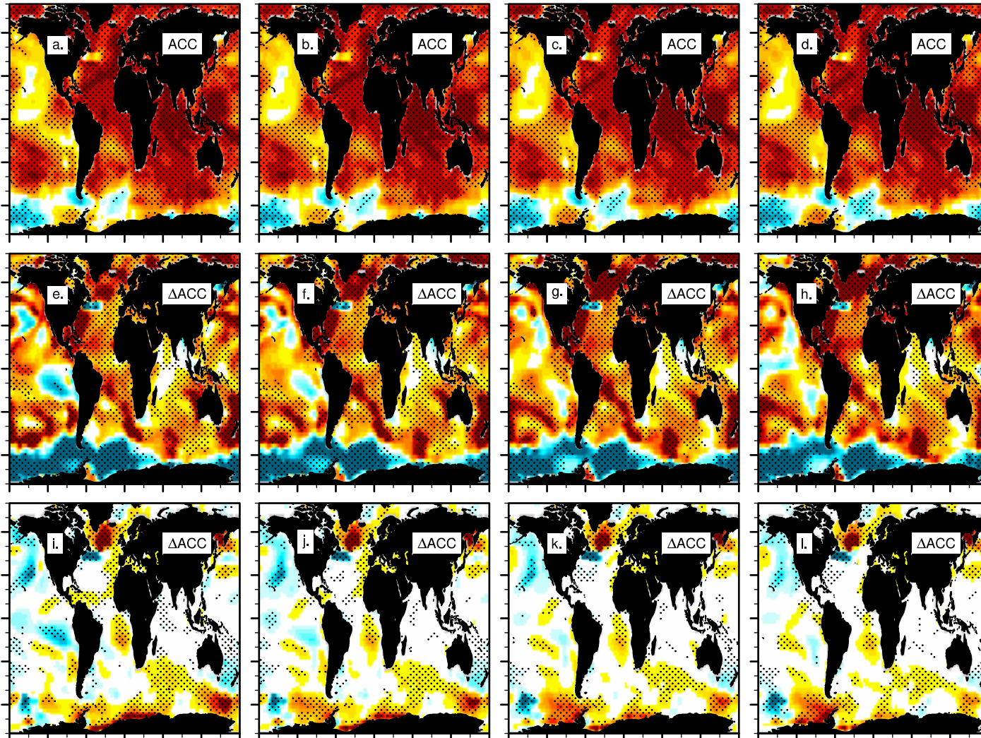
ACC, Sea Surface Temperature, OBS=ERSSTv5, Season=ANNUAL, (LY 3-7: 1959.5-2014.5)
