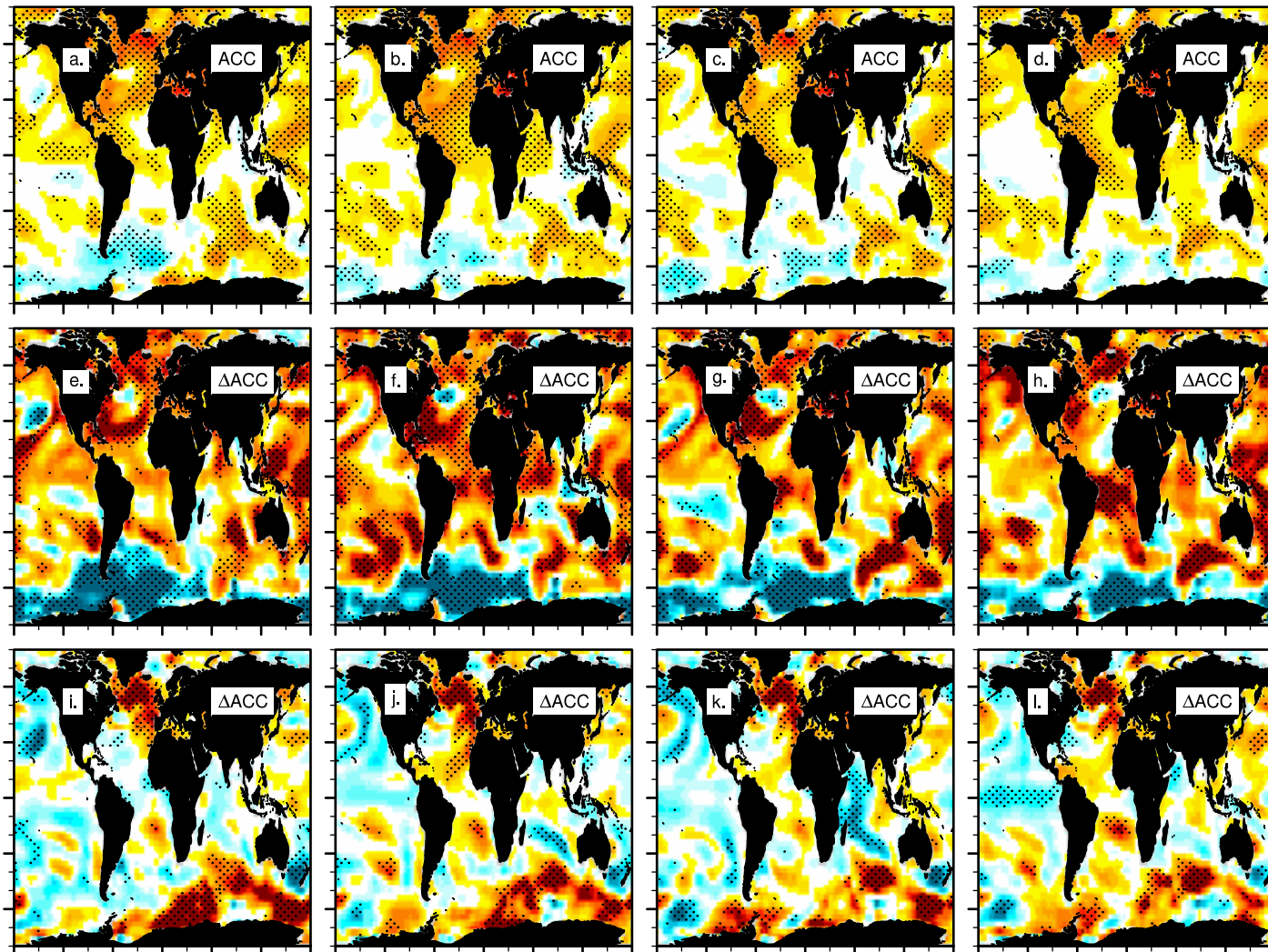
ACC, Sea Surface Temperature, OBS=ERSSTv5, Season=ANNUAL, (LY 5: 1959.5-2016.5), detrended
