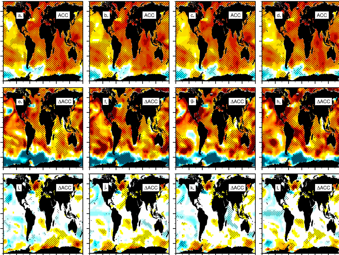
ACC, Sea Surface Temperature, OBS=ERSSTv5, Season=ANNUAL, (LY 5: 1959.5-2016.5)
