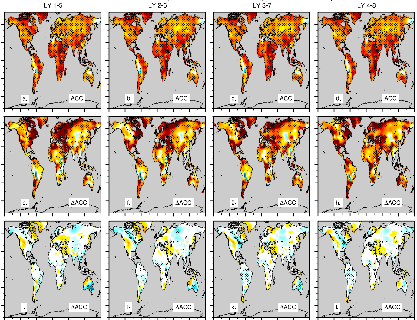
ACC, Surface Air Temperature, OBS=CRU-TS4.0, Season=DJF, (LY 1-5: 1957.0-2013.0)
