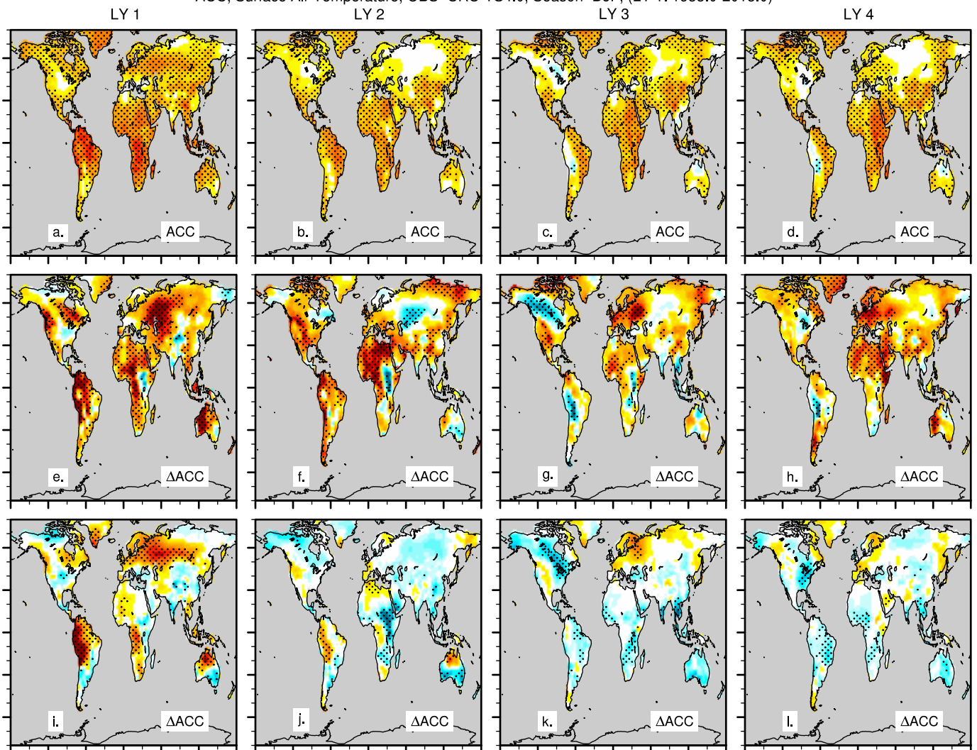
ACC, Surface Air Temperature, OBS=CRU-TS4.0, Season=DJF, (LY 1: 1955.0-2015.0)
