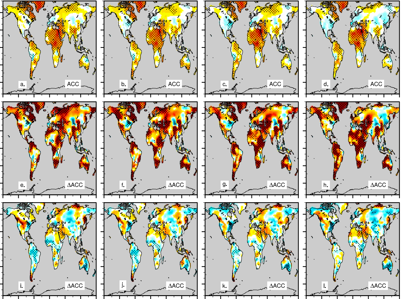
ACC, Surface Air Temperature, OBS=CRU-TS4.0, Season=DJF, (LY 3-7: 1959.0-2013.0), detrended LY 3-7 LY 4-8 LY 5-9 LY 6-10
