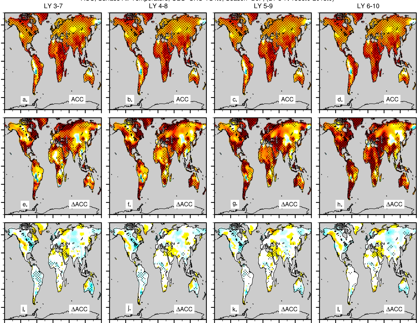
ACC, Surface Air Temperature, OBS=CRU-TS4.0, Season=DJF, (LY 3-7: 1959.0-2013.0)
