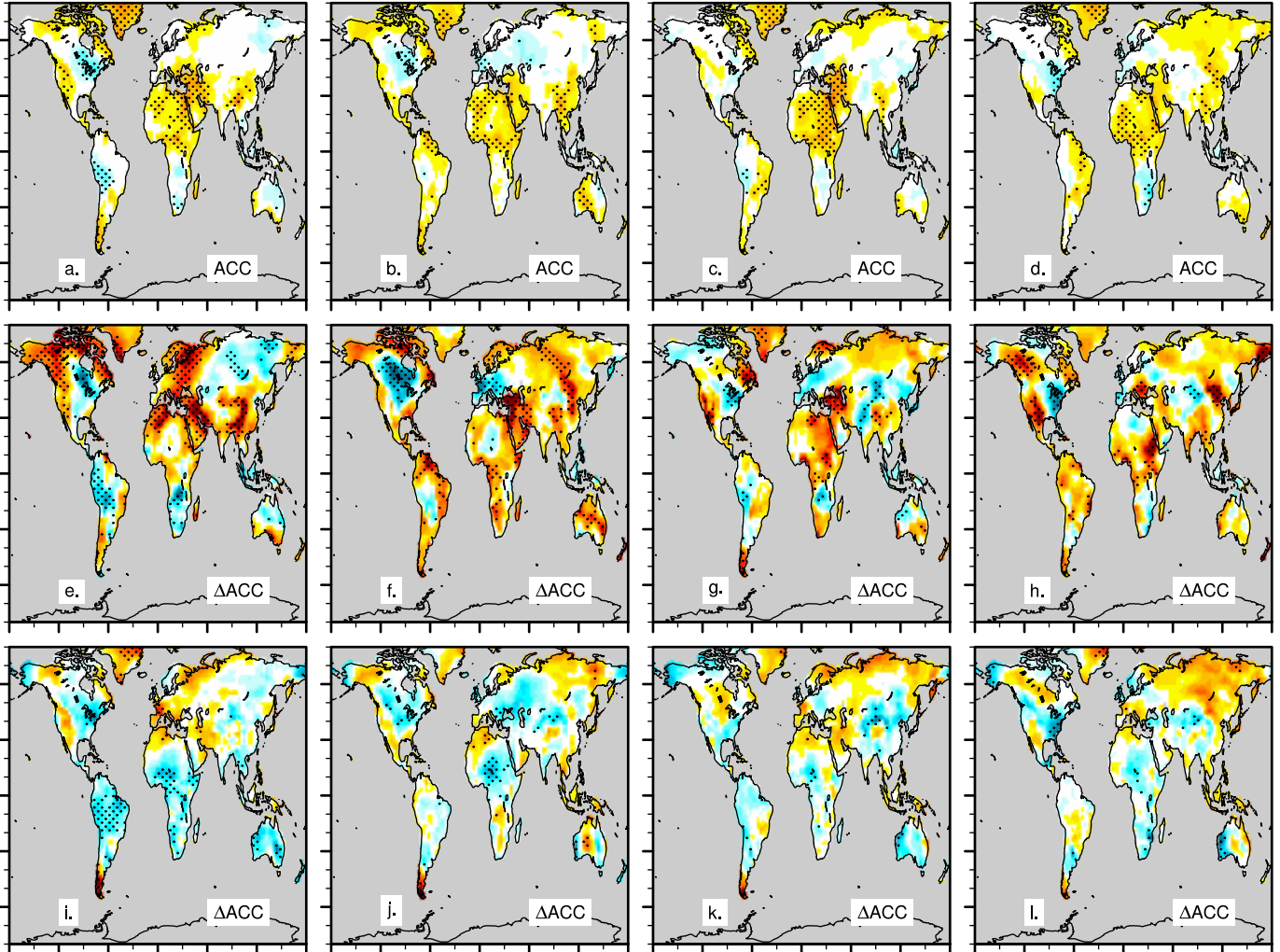
ACC, Surface Air Temperature, OBS=CRU-TS4.0, Season=DJF, (LY 5: 1959.0-2015.0), detrended
