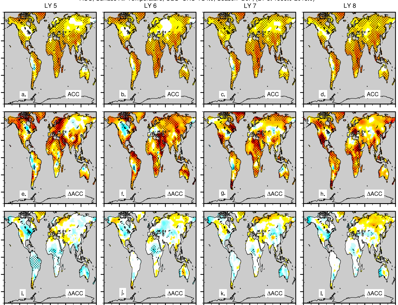
ACC, Surface Air Temperature, OBS=CRU-TS4.0, Season=DJF, (LY 5: 1959.0-2015.0)
