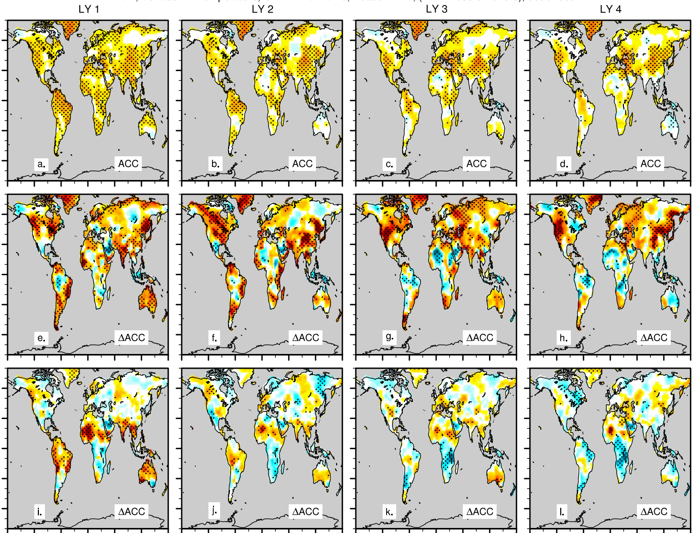
ACC, Surface Air Temperature, OBS=CRU-TS4.0, Season=JJA, (LY 1: 1955.5-2015.5), detrended
