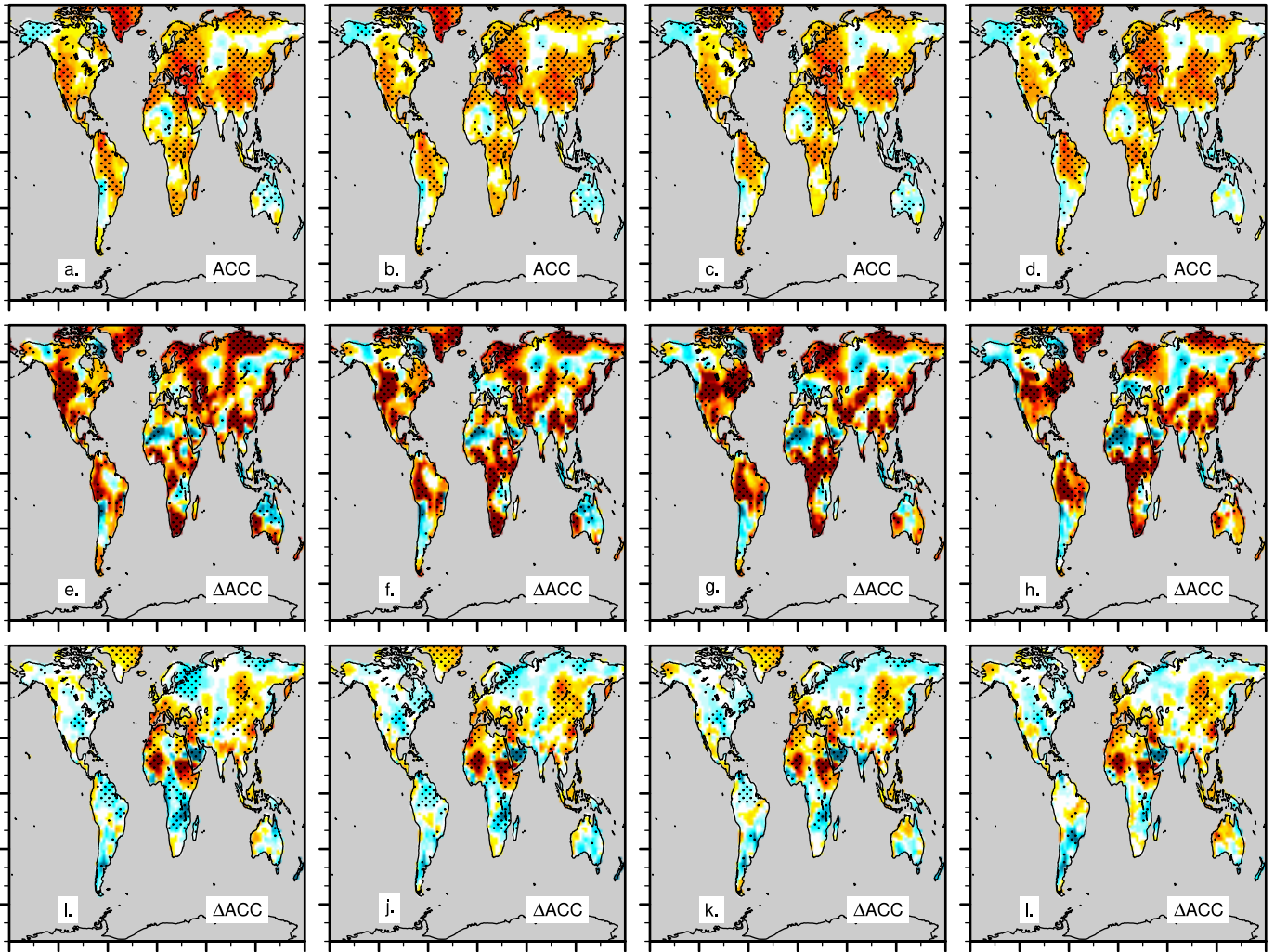
ACC, Surface Air Temperature, OBS=CRU-TS4.0, Season=JJA, (LY 3-7: 1959.5-2013.5), detrended
