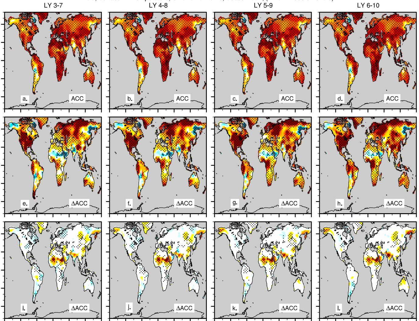
ACC, Surface Air Temperature, OBS=CRU-TS4.0, Season=JJA, (LY 3-7: 1959.5-2013.5)
