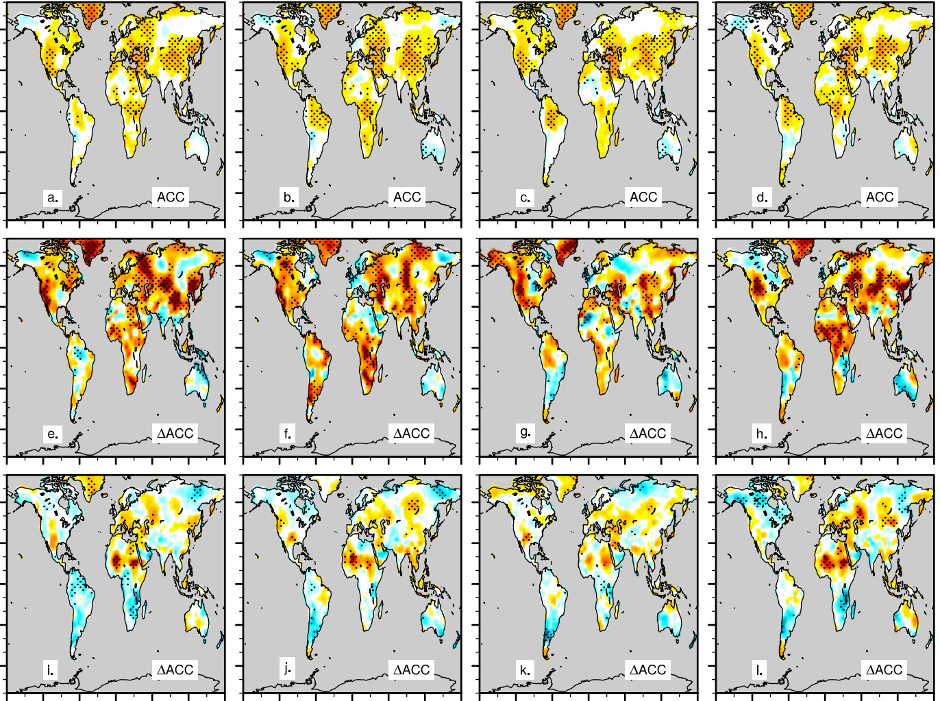
ACC, Surface Air Temperature, OBS=CRU-TS4.0, Season=JJA, (LY 5: 1959.5-2015.5), detrended
