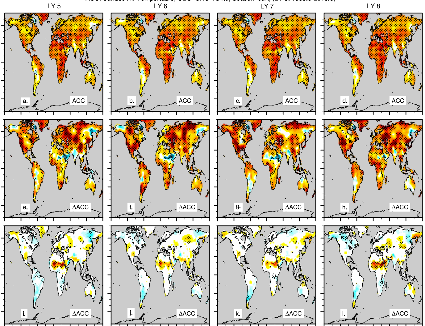
ACC, Surface Air Temperature, OBS=CRU-TS4.0, Season=JJA, (LY 5: 1959.5-2015.5)
