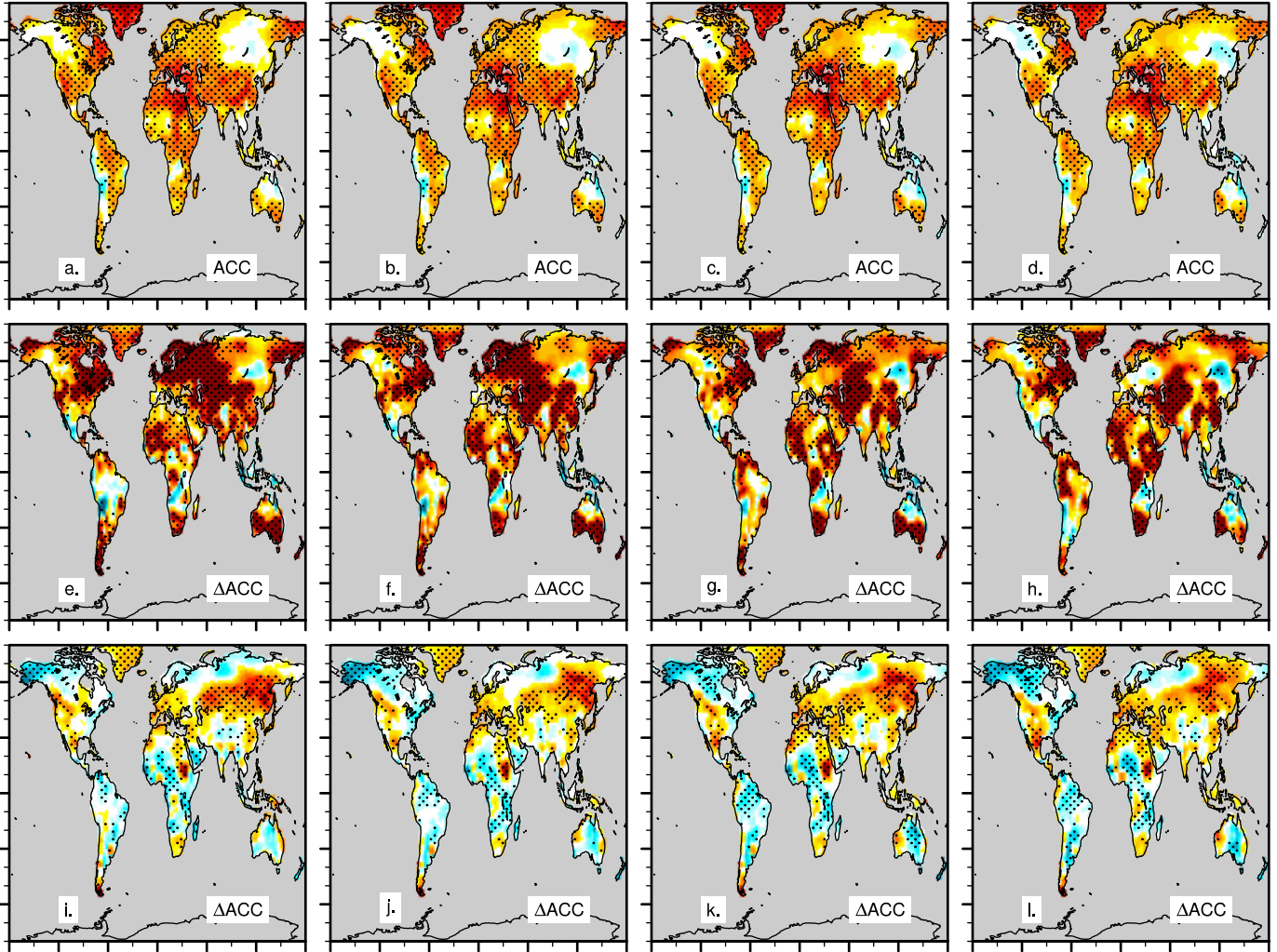
ACC, Surface Air Temperature, OBS=CRU-TS4.0, Season=ANNUAL, (LY 1-5: 1957.5-2013.5), detrended LY 1-5 LY 2-6 LY 3-7 LY 4-8
