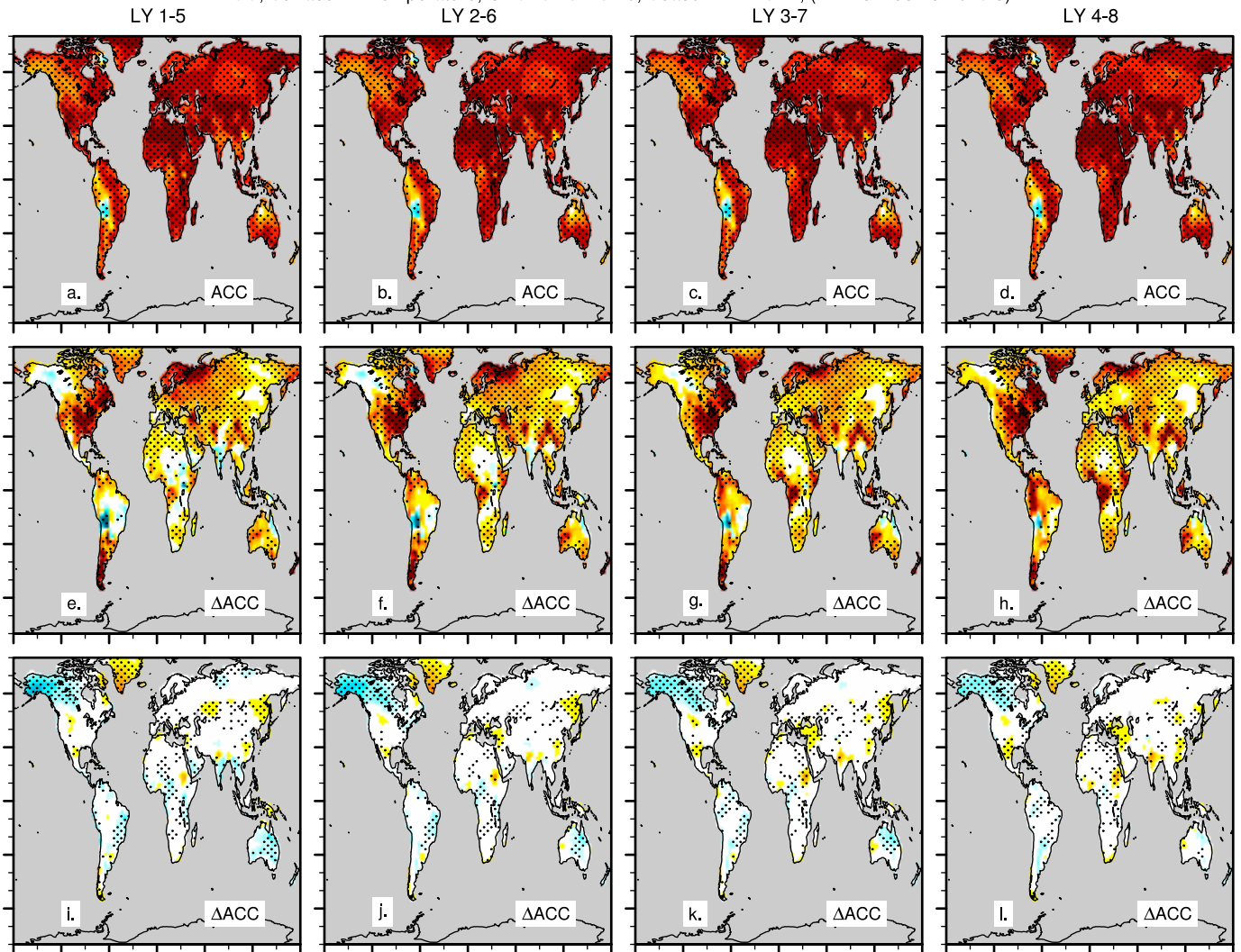
ACC, Surface Air Temperature, OBS=CRU-TS4.0, Season=ANNUAL, (LY 1-5: 1957.5-2013.5)
