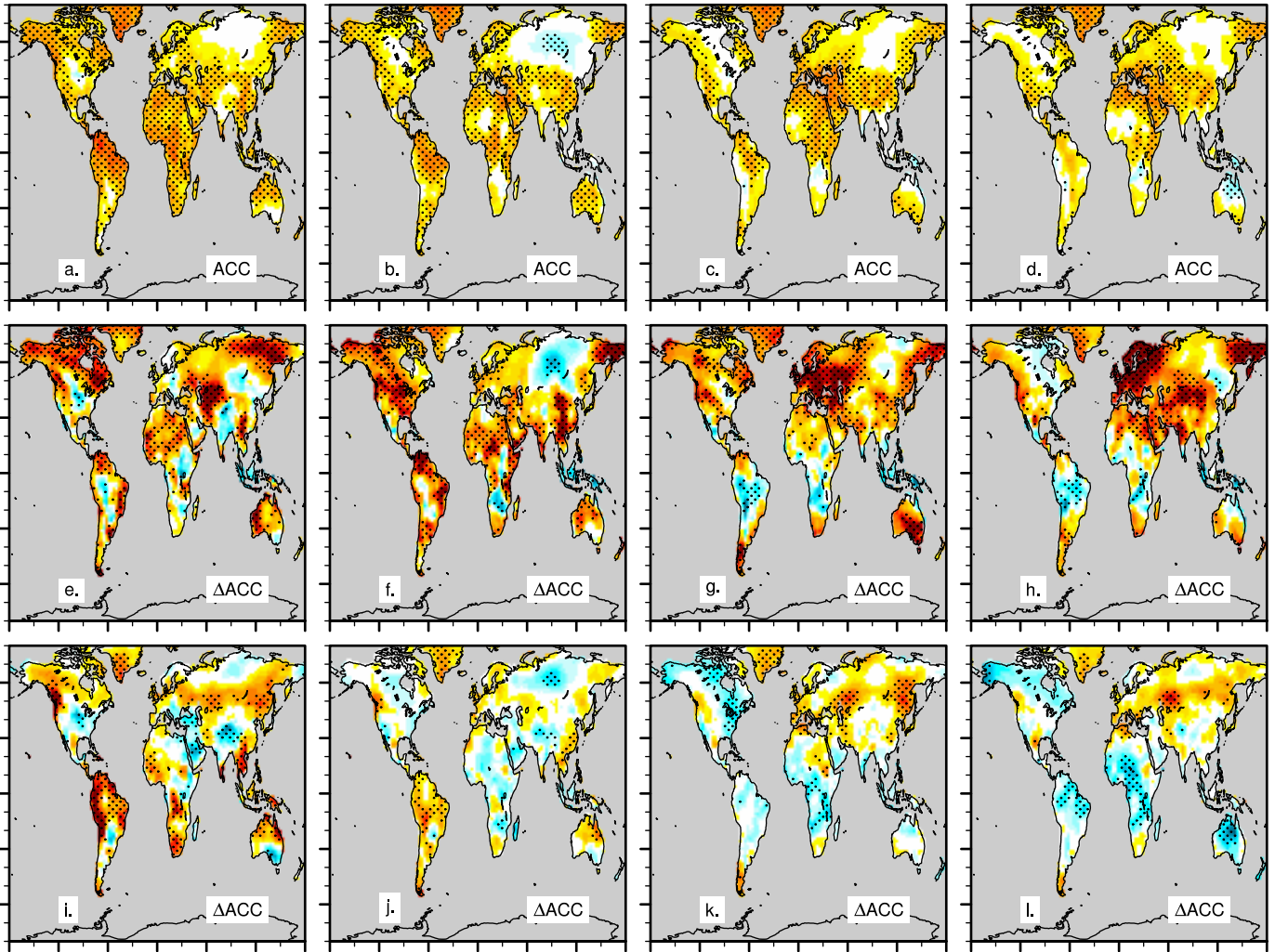
ACC, Surface Air Temperature, OBS=CRU-TS4.0, Season=ANNUAL, (LY 1: 1955.5-2015.5), detrended
