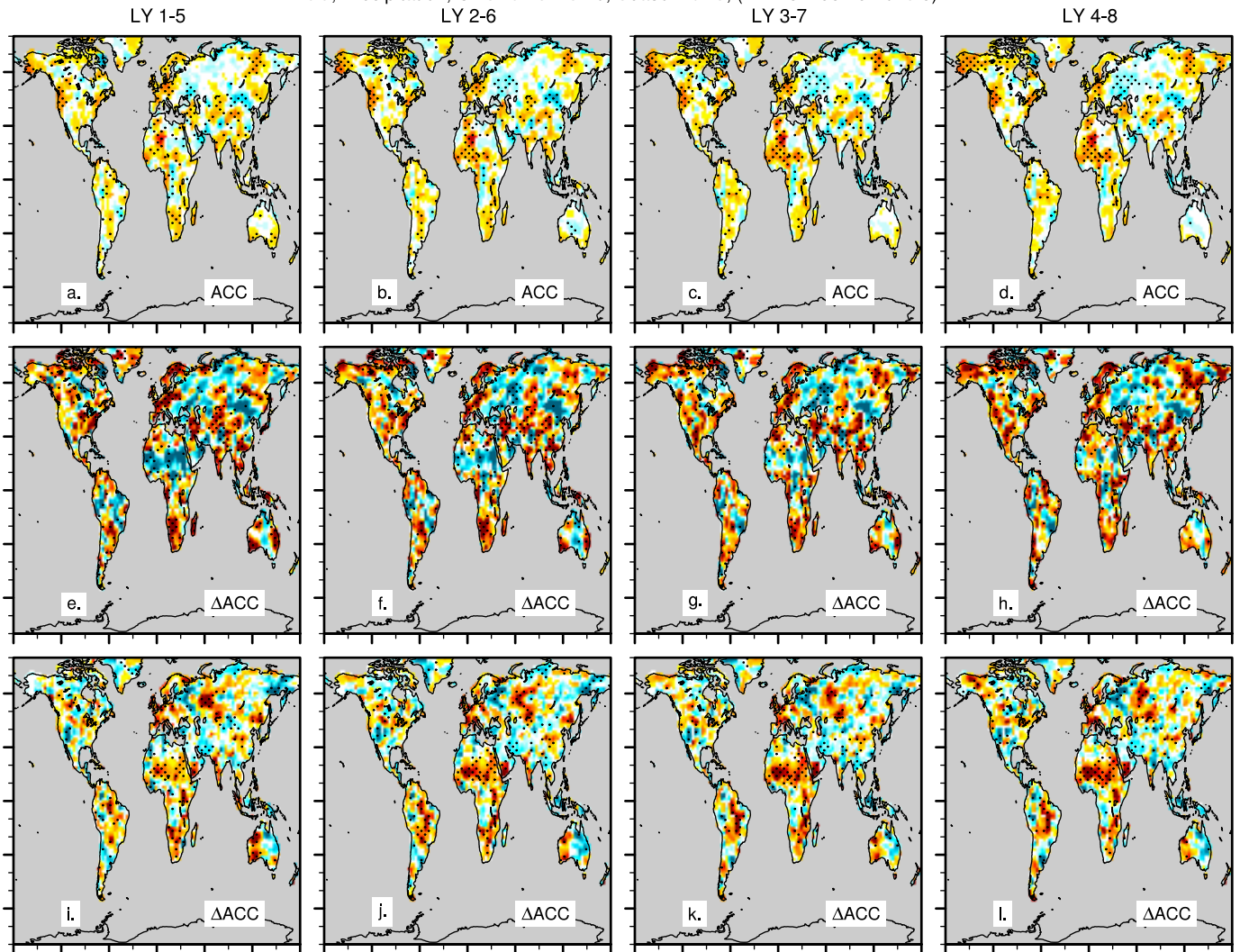
ACC, Precipitation, OBS=CRU-TS4.0, Season=JAS, (LY 1-5: 1957.6-2013.6)
