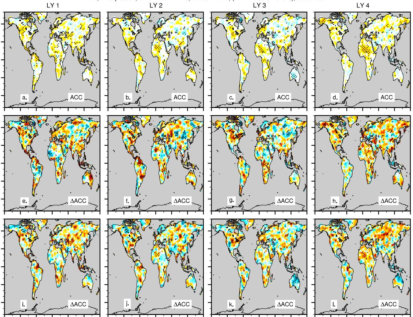
ACC, Precipitation, OBS=CRU-TS4.0, Season=JAS, (LY 1: 1955.6-2015.6), detrended
