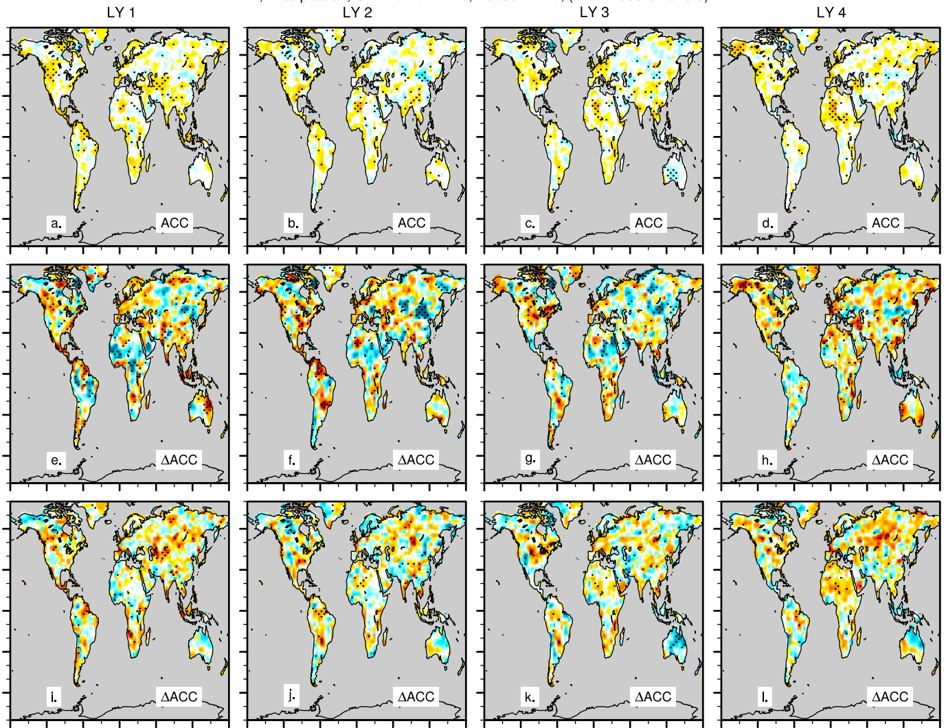
ACC, Precipitation, OBS=CRU-TS4.0, Season=JAS, (LY 1: 1955.6-2015.6)
