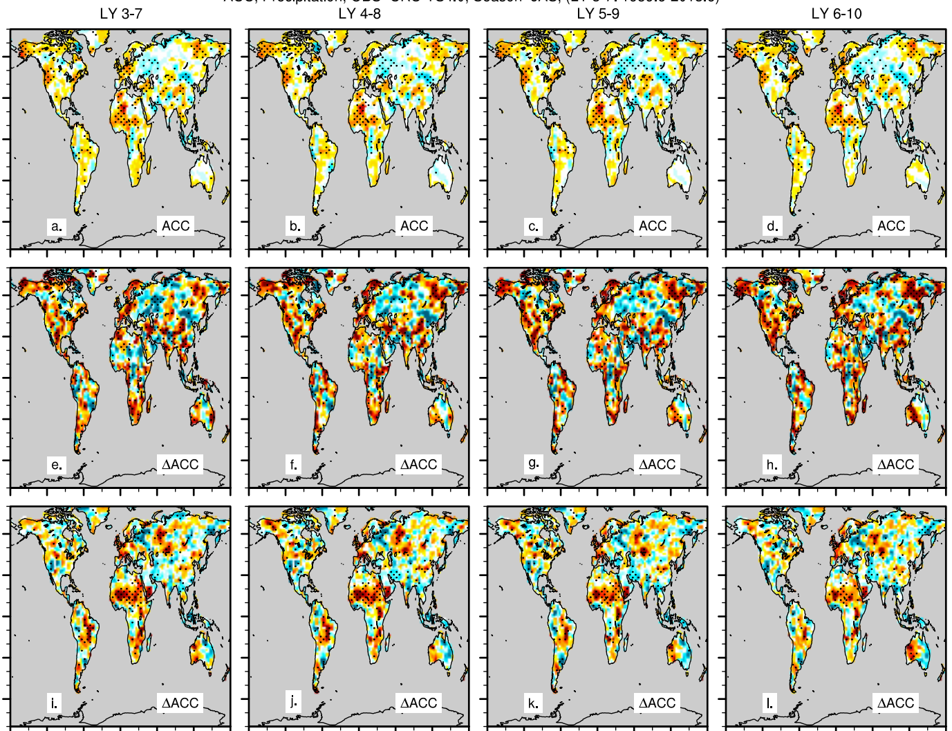
ACC, Precipitation, OBS=CRU-TS4.0, Season=JAS, (LY 3-7: 1959.6-2013.6)
