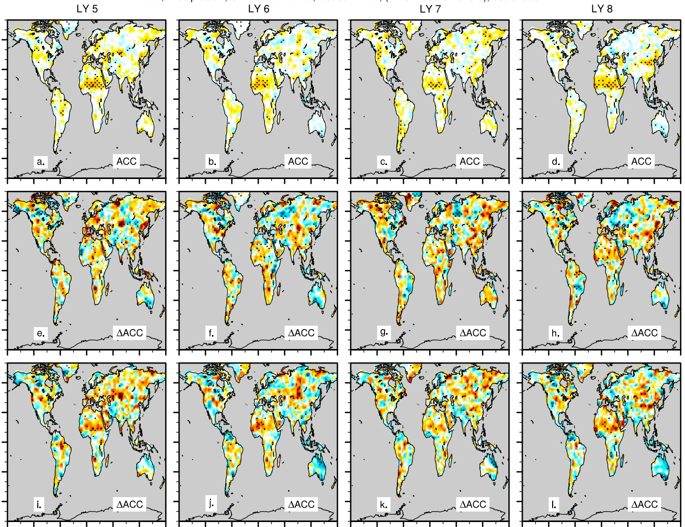
ACC, Precipitation, OBS=CRU-TS4.0, Season=JAS, (LY 5: 1959.6-2015.6), detrended
