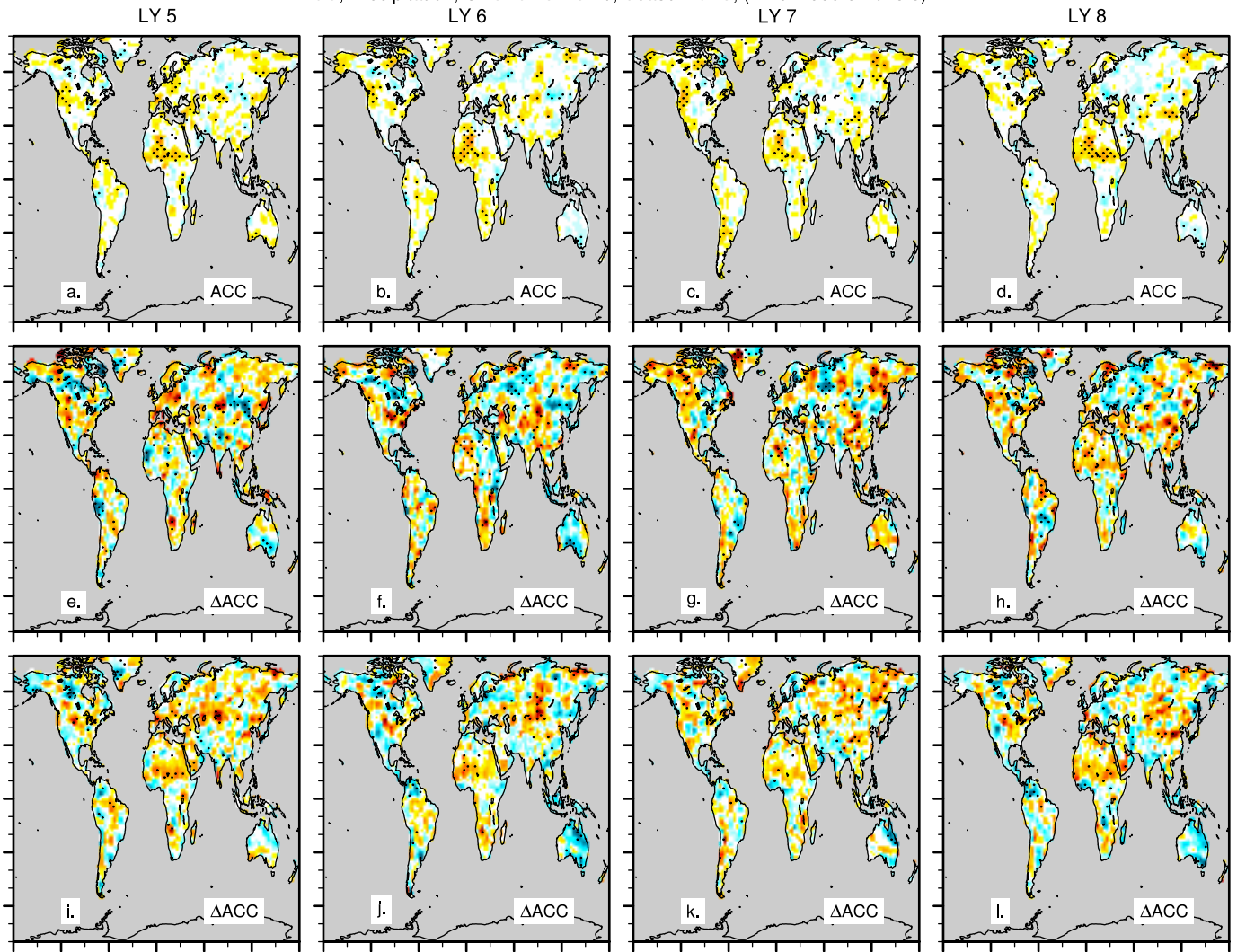
ACC, Precipitation, OBS=CRU-TS4.0, Season=JAS, (LY 5: 1959.6-2015.6)
