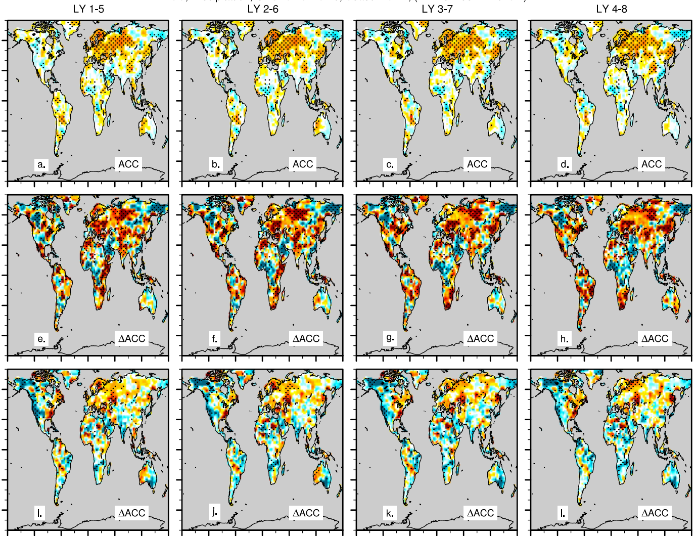
ACC, Precipitation, OBS=CRU-TS4.0, Season=JFM, (LY 1-5: 1957.1-2013.1)
