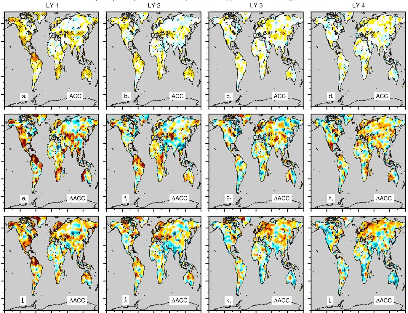
ACC, Precipitation, OBS=CRU-TS4.0, Season=JFM, (LY 1: 1955.1-2015.1), detrended
