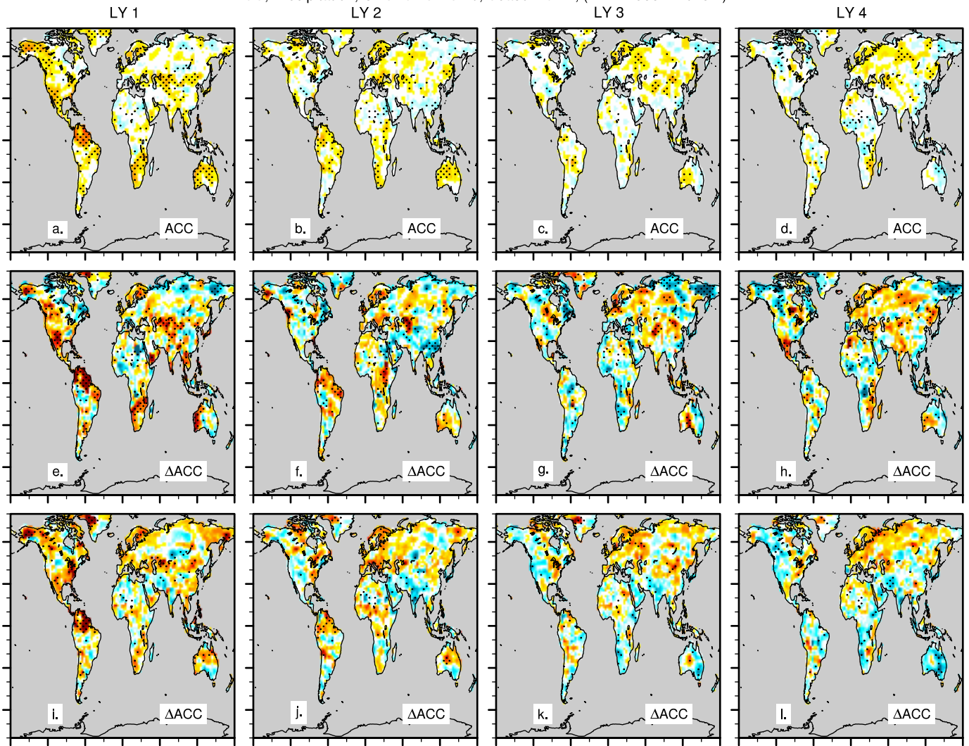
ACC, Precipitation, OBS=CRU-TS4.0, Season=JFM, (LY 1: 1955.1-2015.1)
