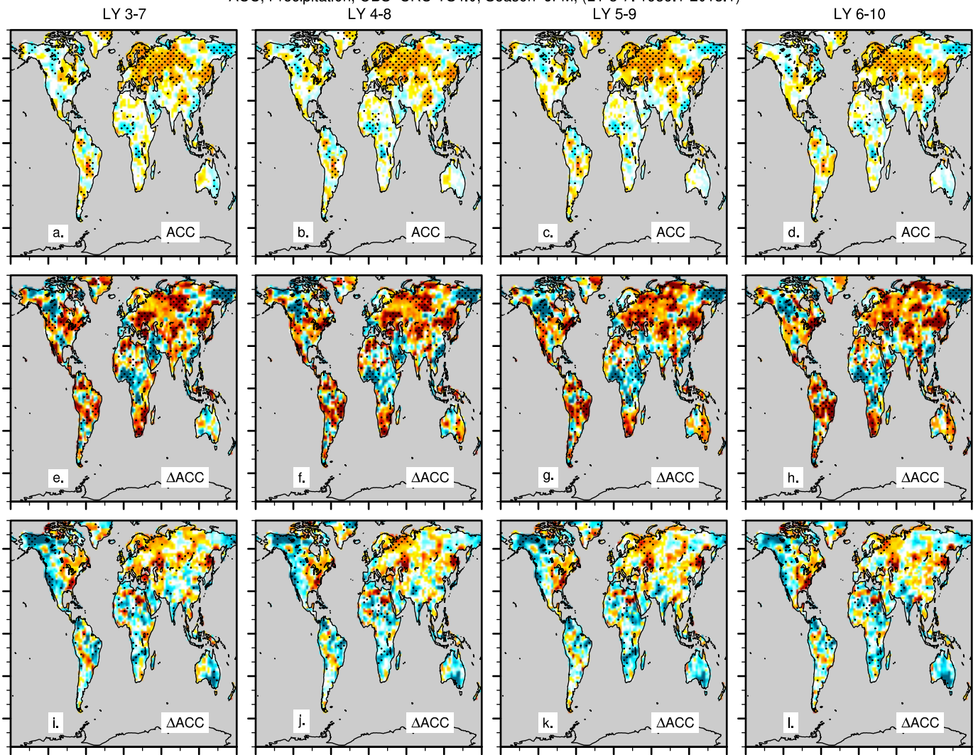
ACC, Precipitation, OBS=CRU-TS4.0, Season=JFM, (LY 3-7: 1959.1-2013.1)
