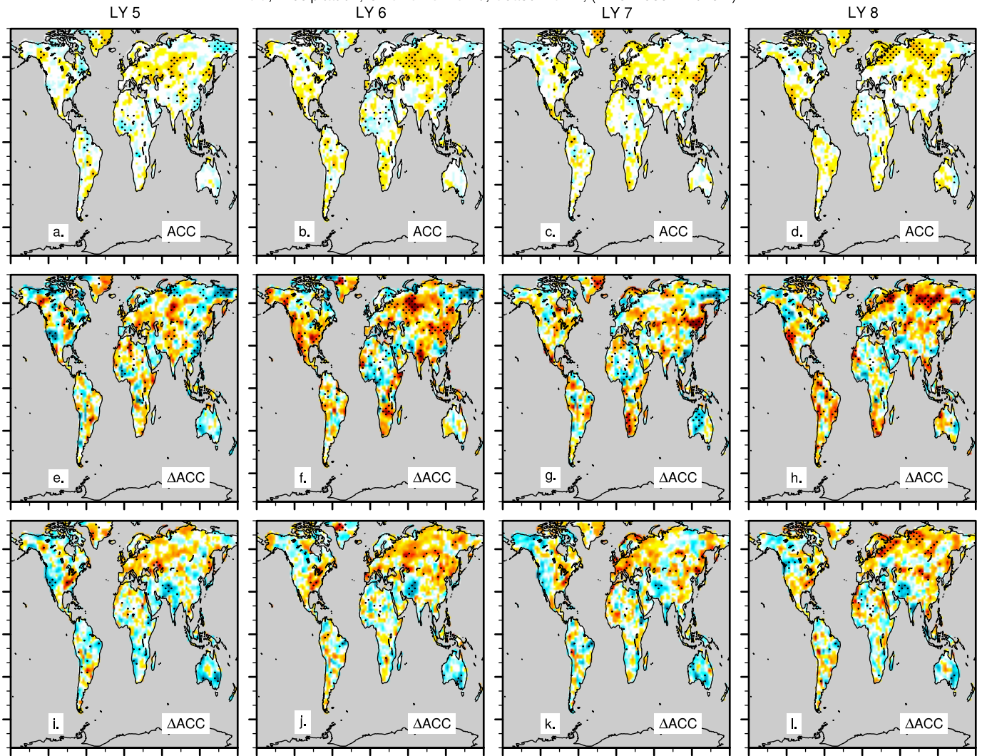
ACC, Precipitation, OBS=CRU-TS4.0, Season=JFM, (LY 5: 1959.1-2015.1)
