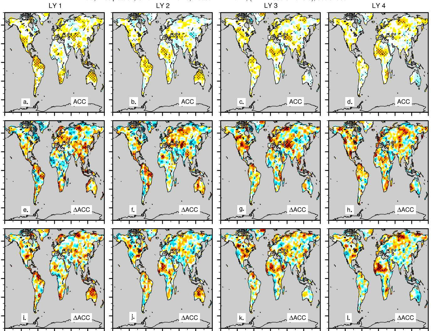
ACC, Precipitation, OBS=CRU-TS4.0, Season=ANNUAL, (LY 1: 1955.5-2015.5), detrended
